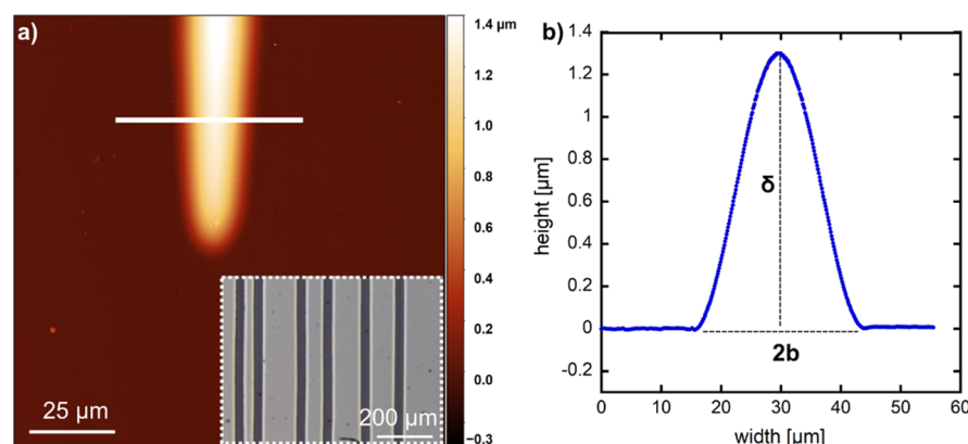
Figure 2. (a) CLSM profile imaging of a spontaneous buckle. Inset shows overview of several straight buckles throughout the sample and (b) buckle height profile corresponding to the region of interest (white line) highlighted in (a) with \delta buckle height and 2b the buckle width indicated.
