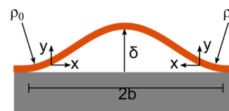
Figure A1. Coordinate system of deflection line y(x) describing the buckled film to determine its radius of curvature at the onset of buckling. Redrawn with modifications after ref 43.
