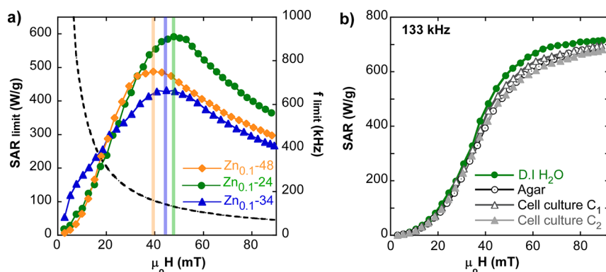
Figure 9. (a) Maximum achievable SAR and \text{SAR}_{\text{limit}} under the Hergt criterion for samples \text{Zn}_{0.1-48}\text{@PEG} , \text{Zn}_{0.1-24}\text{@PEG} , and \text{Zn}_{0.1-34}\text{@PEG} . The black dashed curve is the acceptable maximum frequency, f_{\text{limit}}(H) = 5 \times 10^9/H , for a given magnetic field intensity. The intersection of the black dashed curve and the colored bar of each sample shows the optimal frequency for obtaining the maximum \text{SAR}_{\text{limit}} value. (b) Experimental SAR versus field curves for the \text{Zn}_{0.1-24}\text{@PEG} sample (AC loops in Figure S10, Supporting Information) in aqueous colloid, agar, and cell media at different cell densities ( C_1 and C_2 ; see Section 4).
