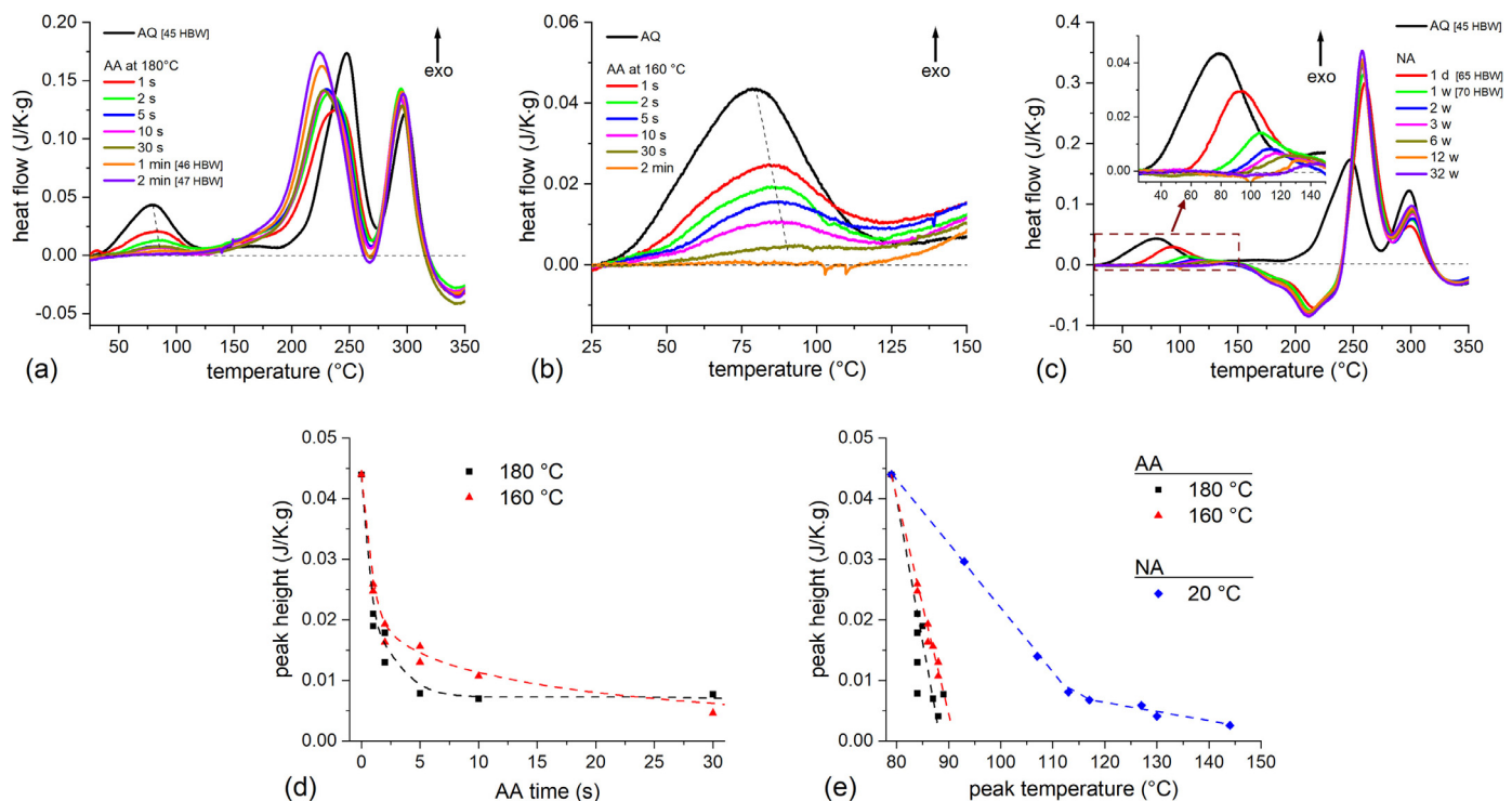
Fig. 2. (a–c) DSC traces measured on alloy 6014 at 10\text{ K}\cdot\text{min}^{-1} directly after quenching ('AQ') and after various pre-ageing treatments at: a) 180^{\circ}\text{C} for 1 s up to 2 min, b) 160^{\circ}\text{C} for 1 s up to 2 min with only the first peak shown, and c) 20^{\circ}\text{C} for up to 32 weeks. Inset in (c) also shows the first peak magnified. Hardness values for some ageing conditions are given in the legends of a) and c). (d, e) Analyses of the first peak in the DSC traces in (a–c): d) Height of the peaks in (a, b) shown as a function of ageing time (including some repeated measurements). e) Height of the peak shown as a function of peak temperature for (a–c).
