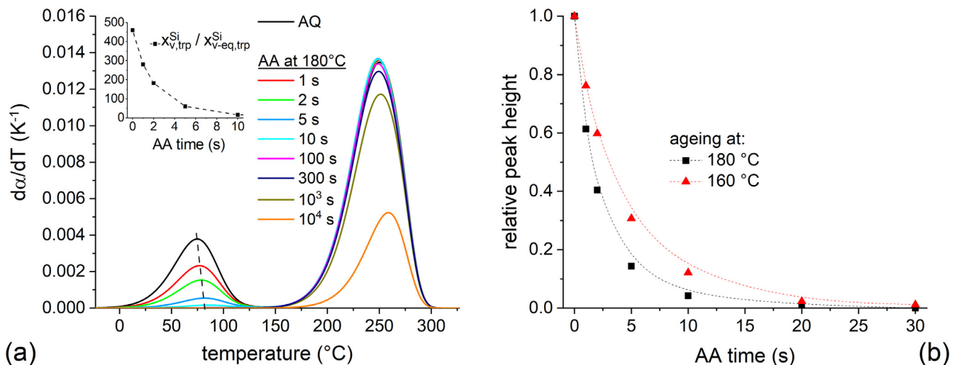
Fig. 6. (a) Calculated d\alpha/dT ('DSC trace'), heating rate 10 \text{ K}\cdot\text{min}^{-1} for as-quenched samples (AQ) and samples aged at 180^\circ\text{C} (AA) prior to DSC. Inset: vacancy site fraction x_{V,\text{trp}}^{\text{Si}} relative to equilibrium value at 180^\circ\text{C} before the DSC run. (b) Height of clustering peak for samples aged at 180^\circ\text{C} and 160^\circ\text{C} relative to peak height in AQ sample.
