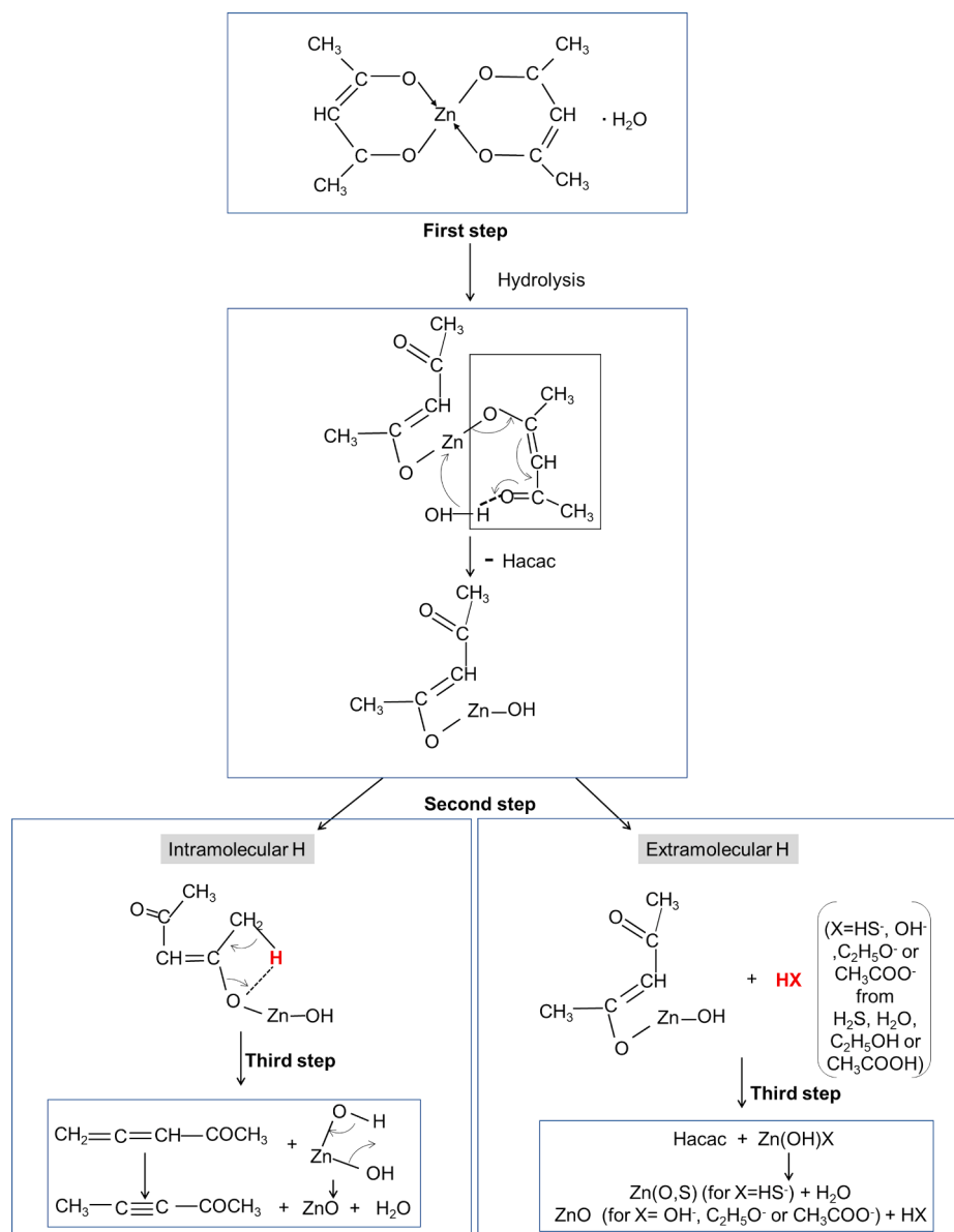
Fig. 5. Scheme of the \text{Zn}(\text{acac})_2 thermal decomposition pathway on the hot substrate. The bond angles and lengths are not drawn to scale.
