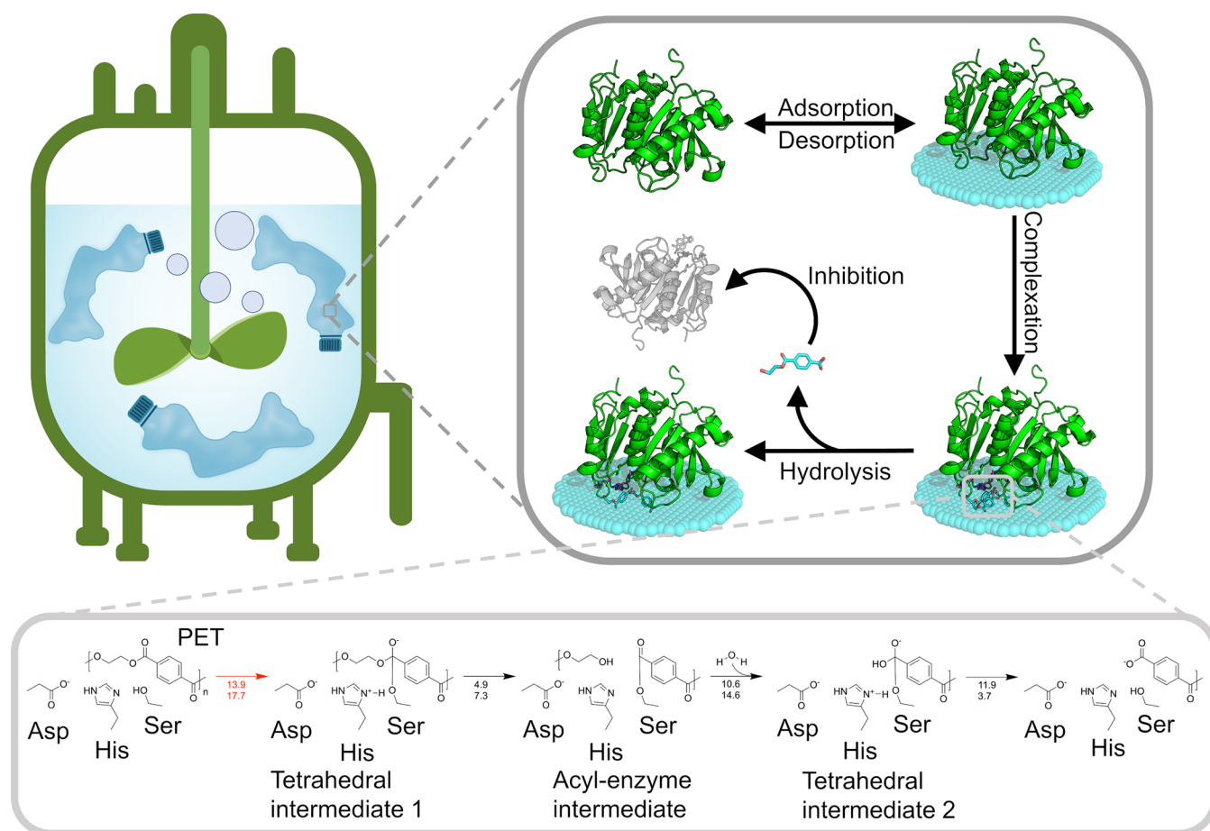
Figure 3. Interfacial biocatalytic hydrolysis of PET and its reaction mechanism. The states of a PET hydrolase are schematically illustrated in the upper right panel. In the lower panel, individual steps of the hydrolysis reaction are schematically shown in line with their activation free-energy barriers in kcal·mol -1 summarized based on different studies. 107,108 The reaction is initiated by a nucleophilic attack by a catalytic serine resulting in a tetrahedral intermediate stabilized by a catalytic histidine, an aspartic acid, and the oxyanion hole, followed by breakdown of the tetrahedral intermediate 1 into an acyl–enzyme intermediate and release of an alcohol. The aspartate–histidine pair activates the water for attack on the acyl–enzyme intermediate carbonyl, resulting in the formation of the second tetrahedral intermediate. The deacylation of this tetrahedral intermediate releases the carboxylic acid product. The rate-limiting step is regarded as the initial nucleophilic attack and highlighted in red with two free-energy activation barriers denoted. The top number is the Boltzmann-weighted average from 20 QM/MM MD simulations, 108 and the bottom number comes from adiabatic mapping studies. 107
