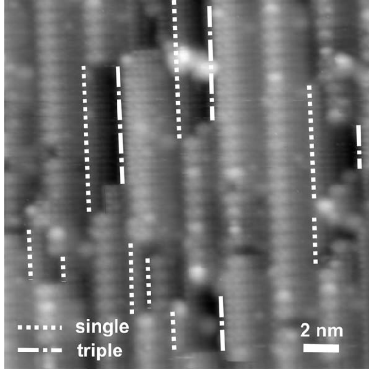
Figure 21: Empty state images ( V_{\text{sample}} = +1.3 V, I_t = 100 pA) of a Si(100) substrate with 6^\circ misorientation in [011] direction after growth of a thin homoepitaxial buffer layer: The irregular step structure is characterized mainly by double-layer steps. Individual single-layer and triple-layer steps are indicated by dotted and dot-dashed white lines, respectively.
