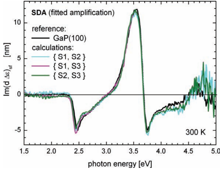
Figure 78: Calculated surface dielectric anisotropy (SDA) of GaP/Si(100) derived by calculation of Eq. 15 for sets of two samples and fit of the output SDA to that of GaP(100) using the APD concentration of the respective samples as fitting parameters.
