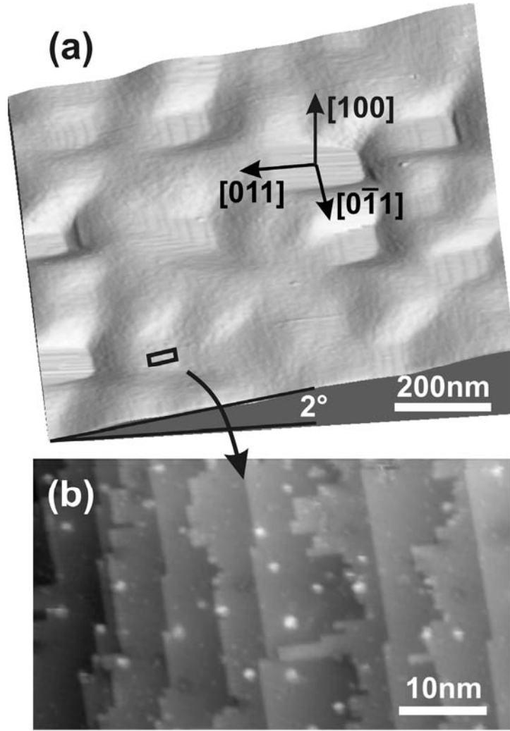
Figure 19: Empty state images of thermally deoxidized Si(100) with 2^\circ misorientation in [011] direction: The large scale image (a) ( V_{\text{Sample}} = +1.2 V, I_t = 60 pA) shows a typical array of terraces separated by rougher regions in-between. In the high-resolution image (b) ( V_{\text{Sample}} = +1.5 V, I_t = 50 pA), the step structure of one of the rougher regions of part (a) is visible in more detail.
