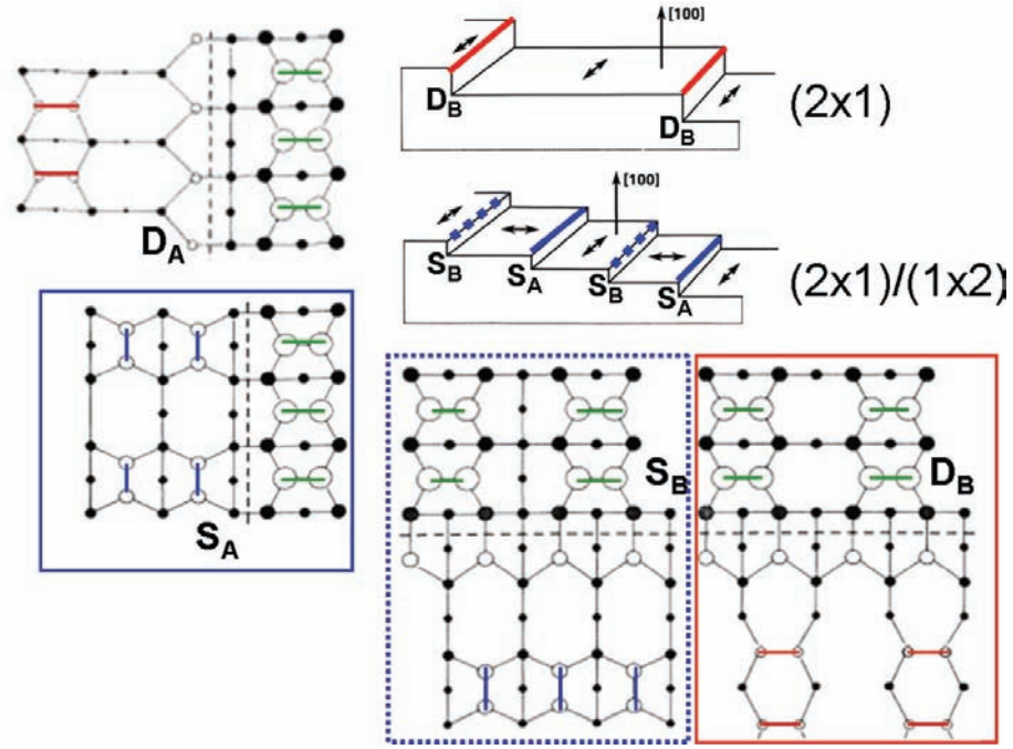
Figure 4: Schematic sketch of the atomic surface structure of Si(100) defining the type of step by the dimer orientation relative to the step edge according to Ref. [36]. Open (filled) circles represent Si atoms of the surface (sub-surface layers), their size indicates relative height. Dimers on the upper terrace are marked by green bars, those one and two atomic layers below by blue and red bars, respectively. Since dimer orientation switches at single-layer steps, both types have to coexist independent of differences in step formation energy, unless the formation double-layer steps of which type B is considered energetically favorable enables a single-domain surface reconstruction.
