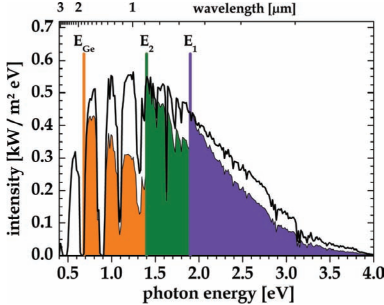
Figure 1: Standard solar spectrum defined by ASTM G-173-03 for terrestrial irradiance considering an effective air mass of 1.5 atmospheres. Colored lines indicate the absorption edges of a typical semiconductor combination applied in current triple-junction solar cells, while the colored area shows an upper limit for the achievable electrical yield only considering transmission below the band gaps and thermalization of the charge carriers to the band edges.
