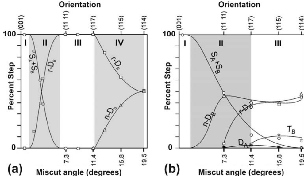
Figure 5: Experimental STM study of the distribution of step types on clean (a) and mono-hydride terminated (b) Si(100) over misorientation angle as reported by Laracuente and Whitman [51]. While double-layer steps prevail on clean vicinal Si(100) beginning with a few degrees off-cut, a significant share of single-layer steps remains present over a wide angular range.
