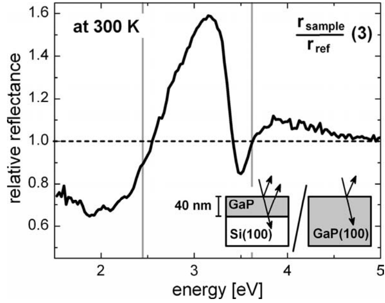
Figure 62: Relative reflectance of the heteroepitaxial GaP/Si(100) sample shown in Figure 61 in relation to the homoepitaxial reference calculated directly from the experimental data according to Eq. 9. The deviations from unity indicate the interference with the interfacial reflection and alter the experimental RA spectra via the normalization of the signal. The gray vertical lines indicate the energetic peak positions of the measured GaP/Si(100) RA spectrum shown in Figure 61.
