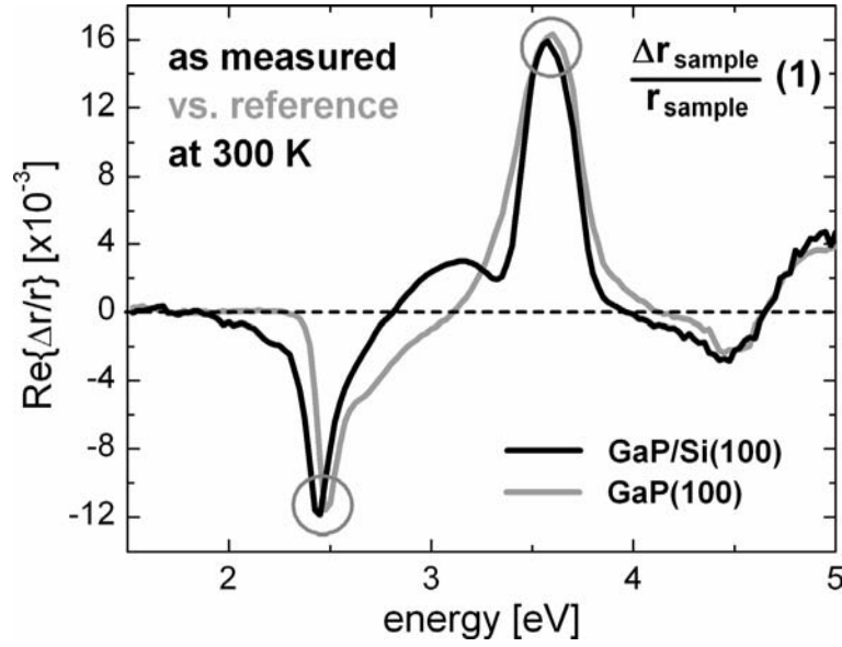
Figure 61: Comparison of the RA spectra measured at an almost single domain heteroepitaxial GaP/Si(100) sample (black curve) and at a homoepitaxially prepared GaP(100) reference (grey). A comparison of the peak heights indicated low anti phase disorder. Differences of the peak intensities indicated an uncertainty of the APD content in the order of a small percentage.
