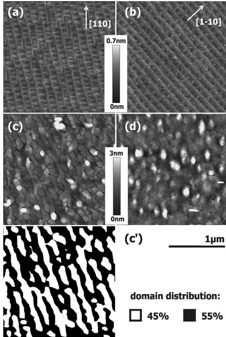
Figure 55: AFM of Si(100) before (a,b) and after GaP/Si(100) growth (c,d): In contrast to sample D (d), the surface of sample S (c) exhibits a network of anti-phase boundaries after GaP/Si(100) growth. In (c') the two different surface domain-types of sample S (c) are color coded in black and white to quantify the surface area covered by each phase.
