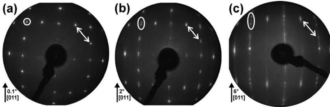
Figure 14: Typical 100 eV LEED patterns observed at Si(100) substrates, misoriented by 0.1^\circ (a), 2^\circ (b) and 6^\circ (c) in the [011] direction, after CVD oxide removal: In (a) and (b), typical half-order diffraction spots in both directions confirmed a two-domain (2 \times 1)/(1 \times 2) surface reconstruction. However, some fine structure due to the periodicity of the step edges also occurred for higher off-cut angles and interferes with evaluation of the domain content, especially in (c).
