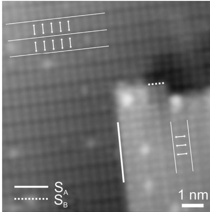
Figure 17: Atomically resolved empty state image ( V_{\text{Sample}} = + 1.3 \text{ V} , I_t = 50 \text{ pA} ) of thermally deoxidized Si(100) with 0.1^\circ misorientation in [011] direction: At the monolayer step, the direction of the Si surface dimers changes. According to the definition of step types, the assignment switches between S_A and S_B where kinks occur, as illustrated in the image.
