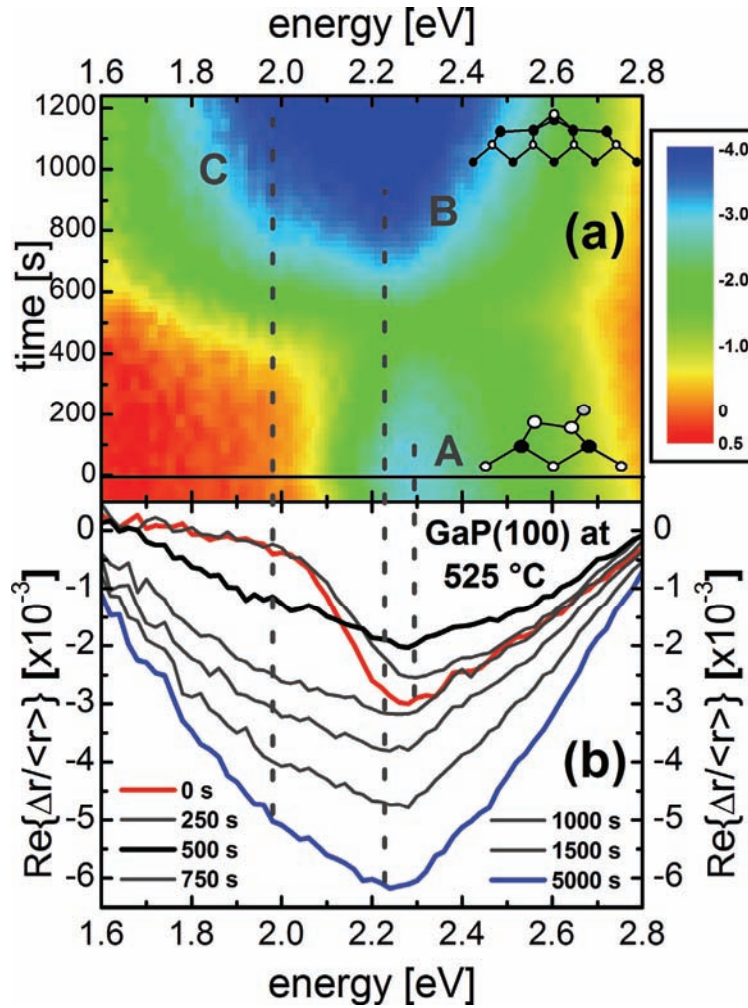
Figure 34: (a) In situ RAS colorplot of a GaP(100) surface at the constant temperature of 525 °C after switch-off of the TBP supply. The measurement focused on the range of the low energy RAS peak at high resolution. The successive transformation from the P-rich to the Ga-rich surface reconstruction is accompanied with specific changes in the peak structure marked by the letters A, B and C. (b) RA spectra extracted from the colorplot at different times. Dashed vertical lines refer to the features observed in the colorplot correlate.
