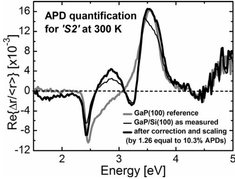
Figure 68: Quantitative in situ RAS analysis of the anti-phase disorder in the GaP/Si(100) film grown on the predominantly single-domain substrate ‘S2’: The measured data (thin black curve) required the correction of interferences via the relative reflectance before linear scaling of the signal (thick black curve) to the intensity of the homoepitaxial reference signal (thick grey curve) eventually resulted in the determination of APD concentration of the sample of about 10.3%.
