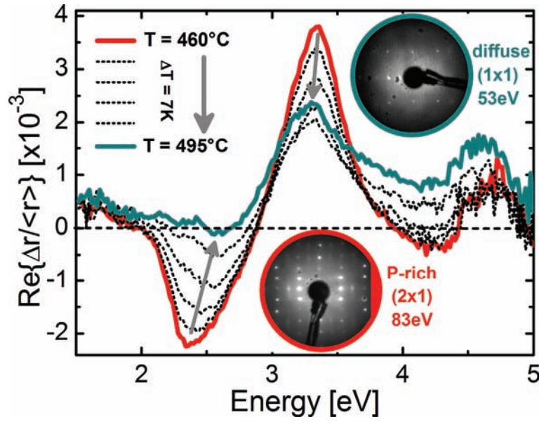
Figure 38: Detailed development of GaP(100) in situ RA spectra during continuous annealing in nitrogen showing the decay of features associated with the initially P-rich surface between 460°C and 495°C in steps of 7K. The insets show LEED patterns of the well-known (2x1)-like surface reconstruction (red, at 83 eV) and of diffuse (1x1) diffraction associated with the intermediate state of the surface (turquoise, at 53 eV).
