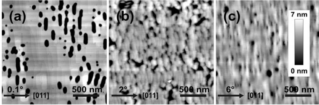
Figure 46: AFM images of the surface of thin heteroepitaxial GaP films grown by MOVPE on Si(100) substrates with different off-cut angles of 0.1° (a), 2° (b), and 6° (c). For the visualization of anti-phase disorder, specific annealing conditions induced preferential desorption at APBs prior to AFM measurement. Due to the choice of contrast for better visibility of surface steps, the complete APD areas appear dark in all images (a-c).
