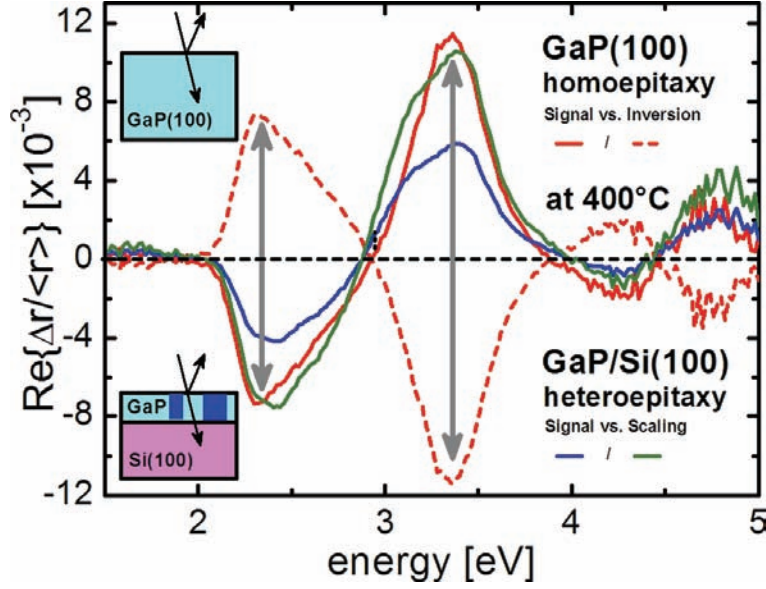
Figure 57: RA spectra extracted from the colorplots presented in Figure 33 (curve with highest peak at 3.4 eV) and Figure 56 (curve with smallest peaks) at 400°C each. The preparation ensured the atomically ordered (2x2)/c(4x2) reconstruction of both surfaces. Regarding the in situ RAS quantification of APD, the spectrum of the homoepitaxial GaP(100) (curve with highest peak) is regarded as reference. Its inversion spectrum (dashed curve) arises when the surface structure is turned by 90°. The curve with smallest peaks represents a GaP/Si(100) layer structure containing APD, which locally turn the surface structure by 90°. It was also scaled up to roughly the amplitude and shape of the reference to provide a scaling factor of m = 1.8 for the APD quantification indicating a concentration of about 22%.
