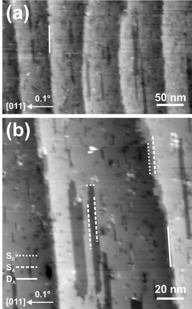
Figure 27: (a) Empty state image of the step structure of a 0.1° misoriented Si(100) surface, which appears to be characterized by double-layer steps of the D A type ( V_{\text{sample}} = 780 mV, I_t = 700 pA). (b) Magnified section of a double layer step, which in most parts consists of an S A step and an S B step, where the intermediate terrace is reduced to a narrow strip, and in some location is missing altogether, resulting in true D A type steps. On the terraces, single layer vacancy islands exist, which are elongated parallel to the terrace edges, leading to long S A type and short S B type vacancy edges ( V_{\text{sample}} = 1240 mV, I_t = 290 pA).
