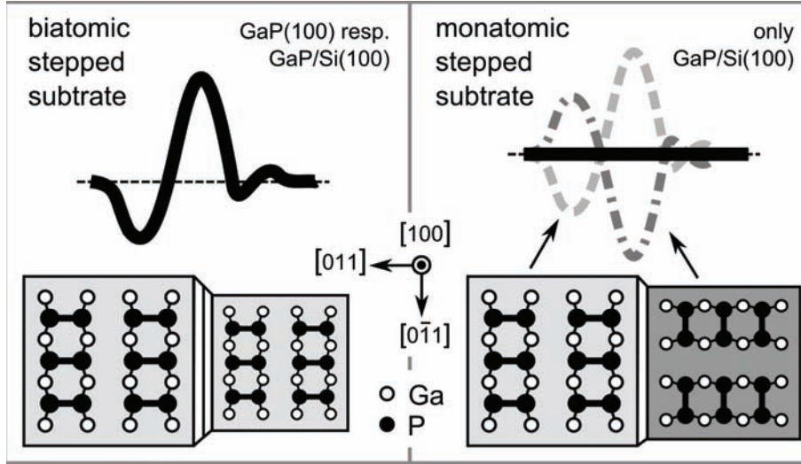
Figure 52: Schematic diagram of P-rich GaP(100) surfaces: The crystal axes define the orientation of the surface reconstruction formed by H-stabilized P-dimers and the sign of the RAS signal. Anti phase disorder causes domains of perpendicular dimer orientation on which the sign of the signal is reversed (right). RAS measurement integrates over macroscopic areas of the surface, effectively resulting in a degradation of the intensity corresponding to the amount of APDs on the surface.
