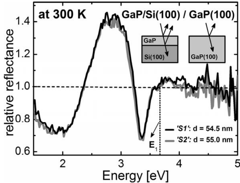
Figure 66: Relative reflectance of heteroepitaxial GaP films grown by the identical process involving conditions for straight APB propagation on different Si(100) substrate of the types ‘S1’ (thin black line) and ‘S2’ (thick grey line). The calculation versus an identically prepared homoepitaxial GaP(100) surface visualizes interferences with the interfacial reflection and allows precise layer thickness determinations by dielectric simulation of the optical response.
