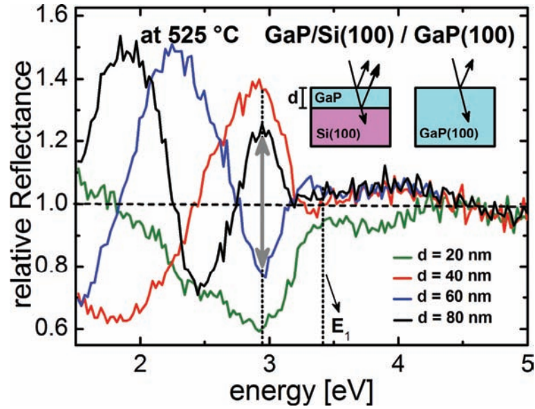
Figure 58: Relative reflectance spectra R_{rel}^{spl}(\lambda) (see text) calculated for the heteroepitaxial growth of a GaP film on a Si(100) substrate in relation to a homoepitaxial GaP(100) reference with identical surface preparation conditions. The individual data sets for different GaP thickness values were taken in growth interruptions with continued TBP stabilization. Due to the optical path difference between the light reflected on the surface and the light reflected at the GaP/Si(100) interface Fabry-Perot interference occurred, which vanished at higher photon energies due to increasing absorption by the GaP film, in particular beyond the E_1 interband transition. Variation of only 20nm film thickness turns a maximum into a minimum and vice versa at around 3eV.
