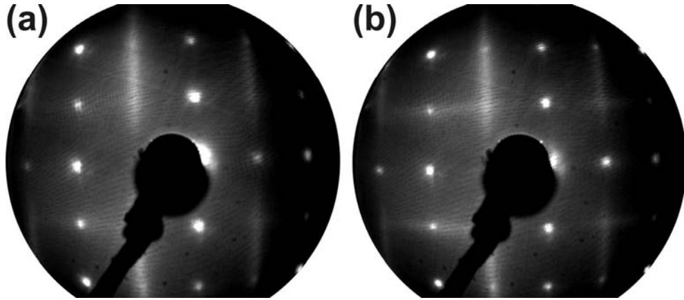
Figure 51: Typical 60 eV LEED patterns measured at heteroepitaxial GaP films grown by MOVPE on 2^\circ off-cut Si(100) substrates. The single-domain surface (a) exactly reproduces the (2x1)-like pattern expected for P-rich prepared GaP(100), while the image of the distinctly two-domain surface (b) contains significant signal of the mutually perpendicular surface reconstruction domain as an indication for the anti-phase disorder in the GaP film.
