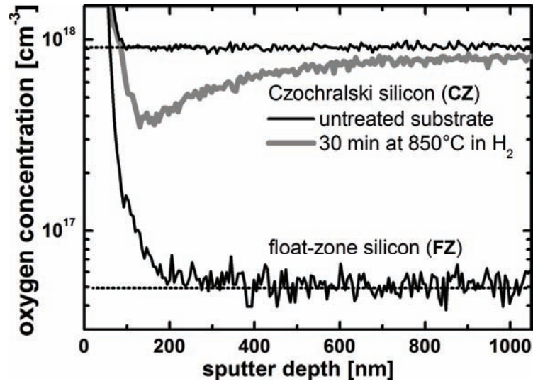
Figure 13: Quantitative SIMS measurements of the oxygen concentration in different Si(100) substrates plotted over sputtering depth. Higher concentrations at the onset of the spectra are due to SiO 2 layers at the surface and the well-known effect of recoil implantation. Higher measurement depths confirm the different intrinsic oxygen concentration levels associated to CZ (top) and FZ (bottom) manufacturing of Si. The curve recorded after thermal annealing in H 2 shows a thermally activated trend for the diffusion of oxygen from the bulk to the surface of the samples.
