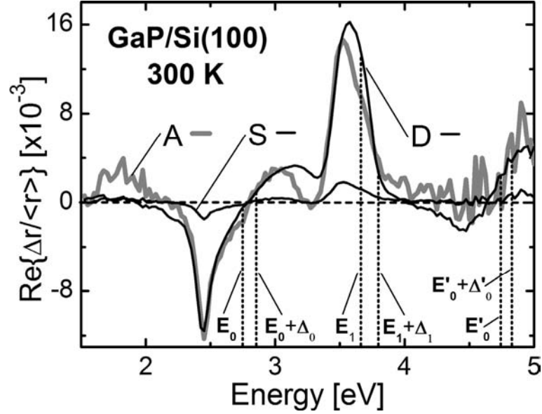
Figure 54: 300K RAS of a single-domain GaP/Si(100) surface (spectrum D ), the corresponding GaP/Si(100) surface that was intentionally prepared as two-domain surface (spectrum S ) and its eightfold amplification (spectrum A ).
