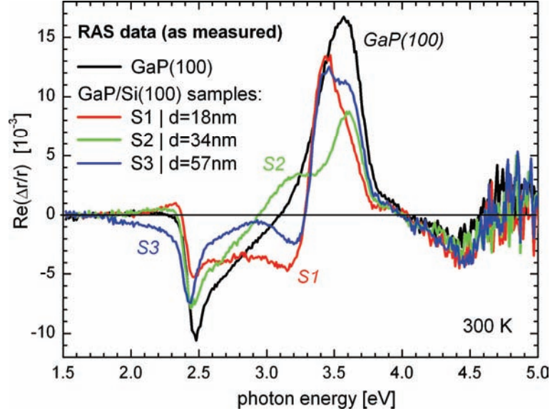
Figure 73: In situ RA spectra of three GaP/Si(100) samples with different GaP film thickness and a homoepitaxial GaP(100) reference. The MOVPE process ensured the formation of a P-rich reconstruction of all surfaces.
