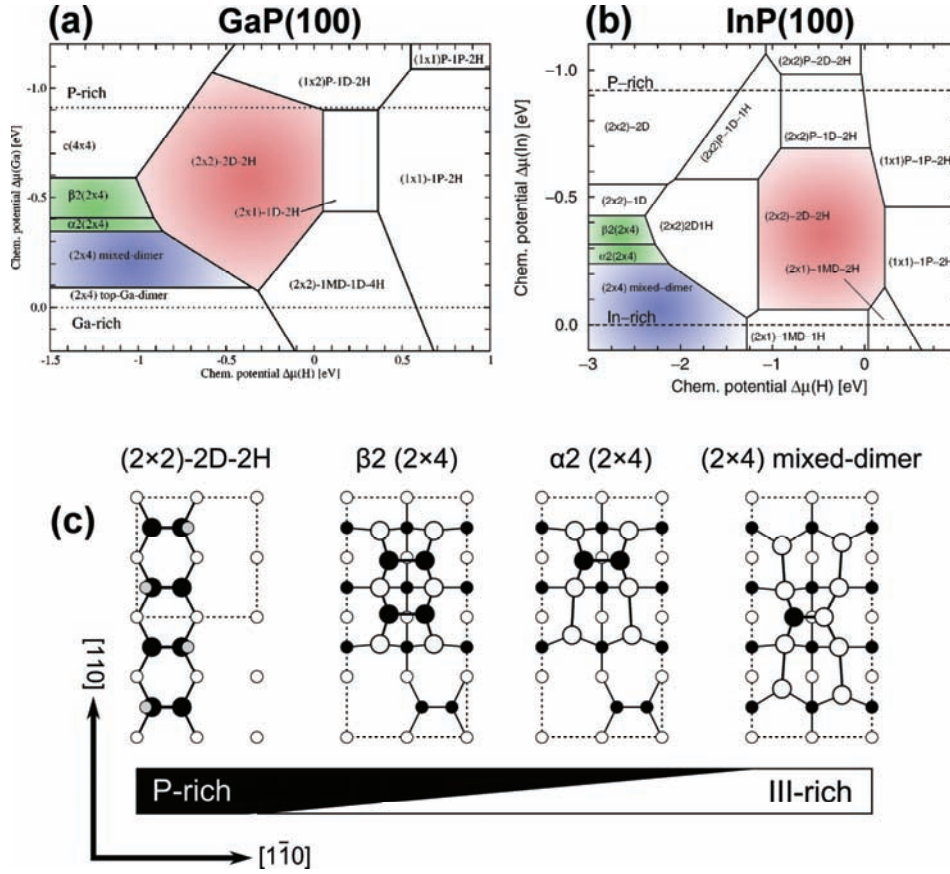
Figure 41: Comparison between the calculated phase diagram of the hydrogen exposed GaP(100) (a) and InP(100) surfaces after Ref. [21] and Ref. [136], where broken lines indicate thermodynamic limitations of the group III chemical potentials and \Delta\mu(\text{H}) is given with respect to molecular hydrogen. Colored areas identify surface reconstructions relevant for this study: the P-rich configuration typical for MOVPE preparation (red), the III-rich mixed-dimer surfaces achievable by annealing without TBP supply (blue), and (2x4) reconstructions with intermediated phosphorus content (green). (c) Top view of the relevant (100) surface reconstruction models ordered with decreasing phosphorus content starting from the hydrogen-stabilized P-rich (2x2)-2D-2H (left), over the intermediate \beta_2(2\times 4) and \alpha_2(2\times 4) to the finally group-III-rich (2x4) mixed-dimer surface (right). According to Refs. [136] and [162], filled (empty) circles represent phosphorus (group-III) atoms and the atomic positions in the uppermost two layers are identified by larger symbols.
