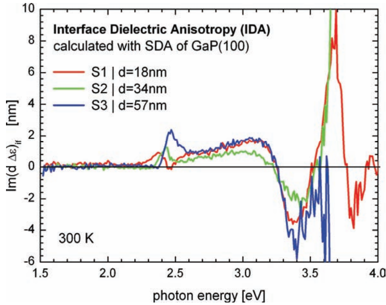
Figure 80: Calculated interface dielectric anisotropy (IDA) of the individual GaP/Si(100) samples shown in Figure 73. The IDAs were derived by solving Eq. 15 using the GaP(100) reference SDA, individual RAS spectra of the respective samples and the derived amplification factors as input parameters. Due to excessive noise in the IDAs caused by absorption above the critical point energy of GaP at about 3.7 eV, the data is only shown up to 4.0 eV and two spectra (green and blue) had to be cut even earlier.
