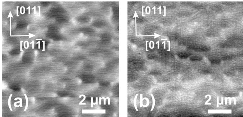
Figure 18: AFM images of deoxidized Si(100) surfaces: Both substrates were 0.1^\circ misoriented towards [011] , but prior to thermal oxide removal in \text{H}_2 they were covered either with a wet-chemical protective oxide layer (a) or with the native oxide of the wafer (b).
