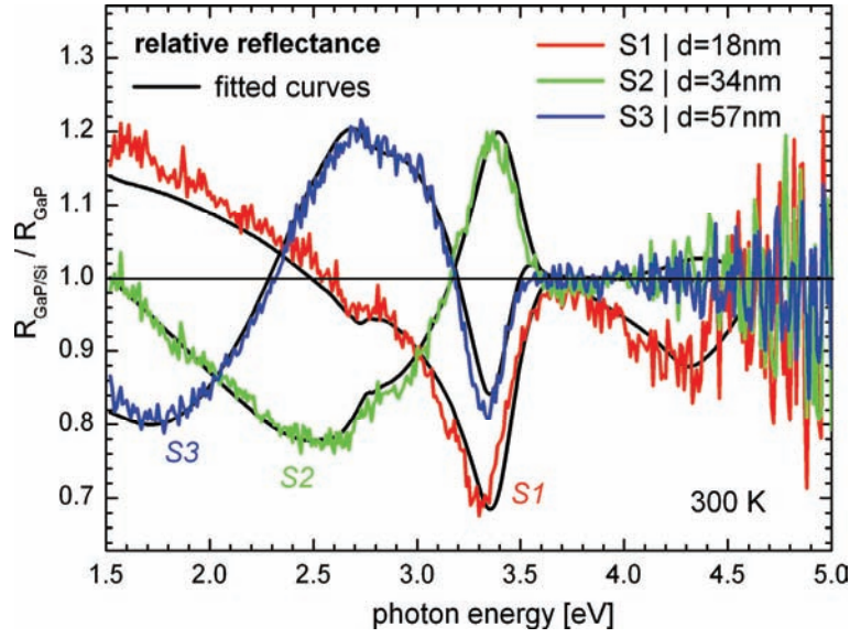
Figure 74: Experimental relative reflectance spectra derived from the data set shown in Figure 73 (colored lines) and thickness dependent fit by an optical model (black lines).
