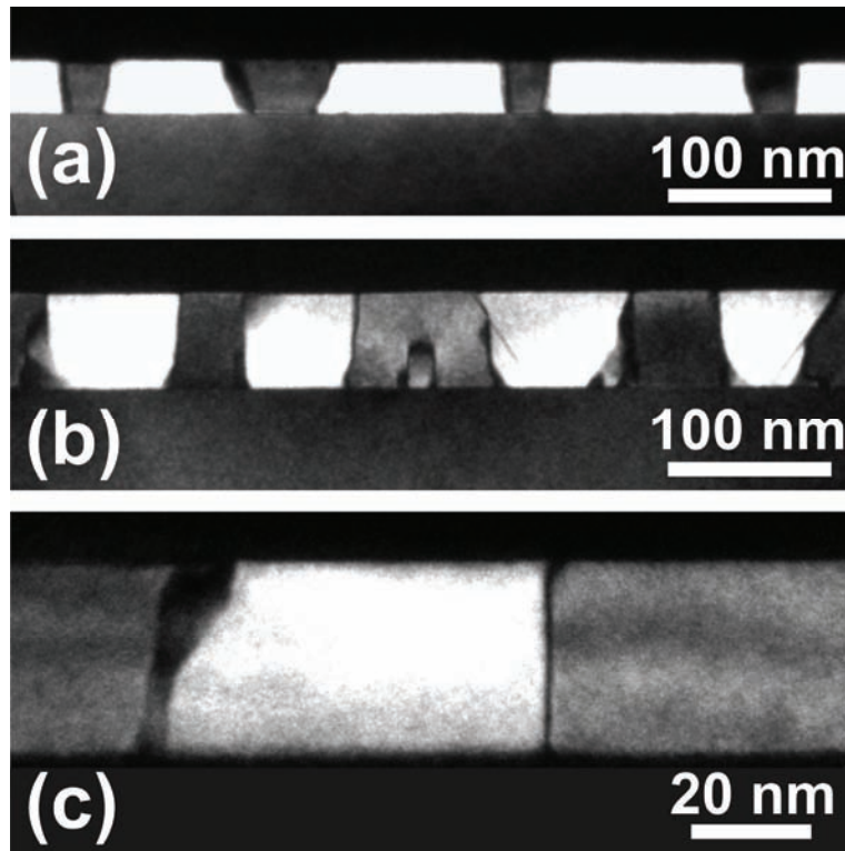
Figure 48: Cross-section TEM images with specific dark-field contrast for visualization of anti-phase disorder. According to the choice of imaging conditions, either the main phase (a) or the APDs (b) can appear bright. Magnification of a single APD (c) shows the difference between the APBs at both edges.
