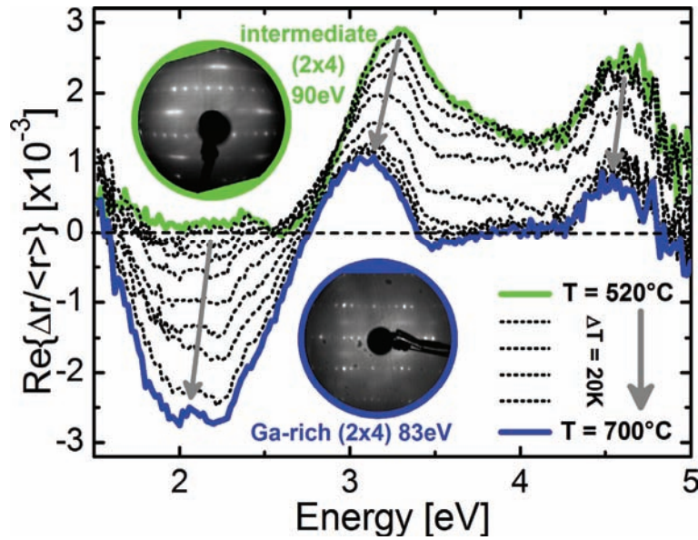
Figure 39: Detailed development of GaP(100) in situ RA spectra during continuous annealing in nitrogen showing the successive formation of features associated with the Ga-rich surface between 520°C and 700°C in steps of 20K. The insets both show LEED patterns with (2x4) symmetry, one measured after annealing in N 2 at 520°C (green, 90 eV), the other after standard preparation of the Ga-rich surface reconstruction (blue, 83 eV).
