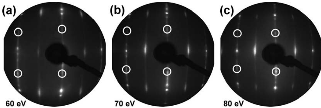
Figure 15: Typical LEED patterns observed at the Si(100) substrate of Fig 1(c) with 6^\circ misorientation in the [011] direction with incident beam energies of 60 eV (a), 70 eV (b), and 80 eV (c): The expected positions for half-order diffraction spots in the [011] direction are indicated by white circles.
