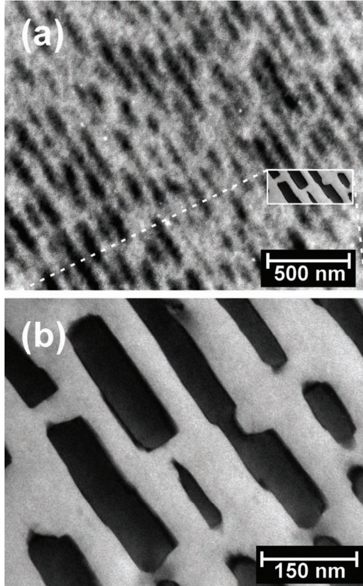
Figure 72: Comparison of a typical LEEM image (a) with a plan-view TEM image (b) of the same GaP/Si(100) sample, both in a respective dark-field mode for the observation of anti-phase disorder. The inset in (a) shows a section of the properly scaled TEM image (b) superimposed on an arbitrarily selected area of the LEEM image for comparison of the imaged structures.
