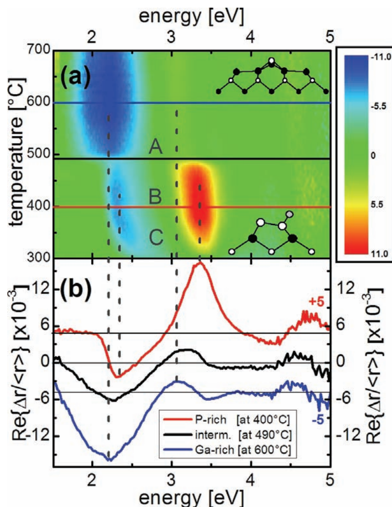
Figure 33: (a) Color-coded representation of a continuous in situ RAS measurement (color-plot) at a GaP(100) surface while the sample temperature was ramped up from 300 to 700°C at a rate of 1.5 K/min without TBP supply. Between 300°C and 490°C, spectra associated with a P-rich surface reconstruction were observed, while beyond 500°C, a Ga-rich reconstruction appeared. In a narrow range around 490°C - 500°C, RA spectra of an intermediate surface reconstruction were taken. Letters mark regions where the development of the RA signal is predominantly caused by changes of the surface reconstruction (A), of the measurement temperature (B) and of the atomic order of the surface (C), respectively. (b) RA spectra representing two well-defined surface reconstructions, the P-rich (2x2)/c(4x2) at around 400°C (upper curve) and the Ga-rich (2x4) at around 600°C (lower curve), were extracted, and also the RA spectrum of the intermediate surface (middle) at ca. 490°C. Dashed vertical lines at the peak positions refer to the respective features in the colorplot.
