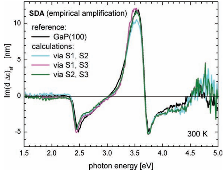
Figure 77: Calculated surface dielectric anisotropy (SDA) of GaP/Si(100) derived by calculation of Eq. 15 for sets of two samples and input of empirical APD amplification factors in comparison to the reference SDA of GaP(100).
