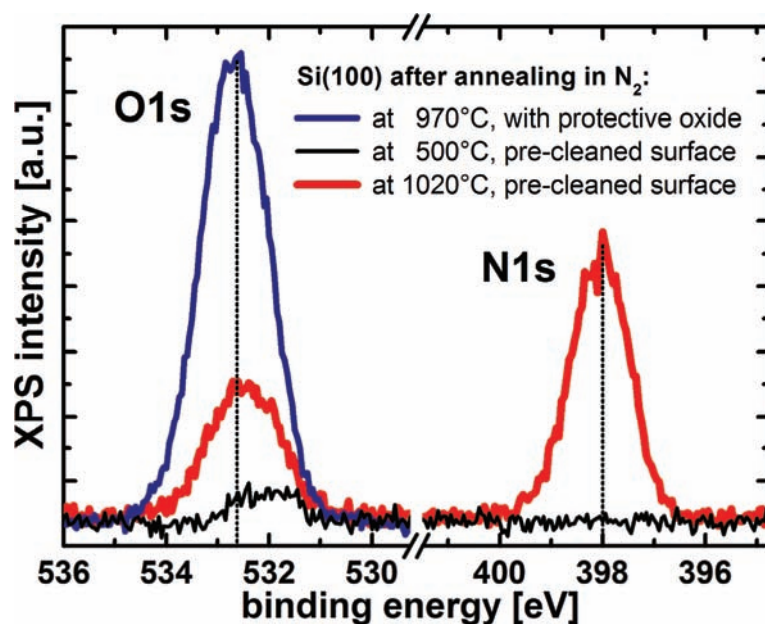
Figure 11: O1s and N1s photoemission lines measured at three Si(100) substrates which were annealed in nitrogen at a pressure of 950 mbar: Two sample were previously cleaned in a hydrogen ambient and then annealed in N_2 at surface temperatures of about 500°C (thin black) and 1020°C (thick red), respectively, while another one was annealed at 970°C exclusively in N_2 process gas (blue).
