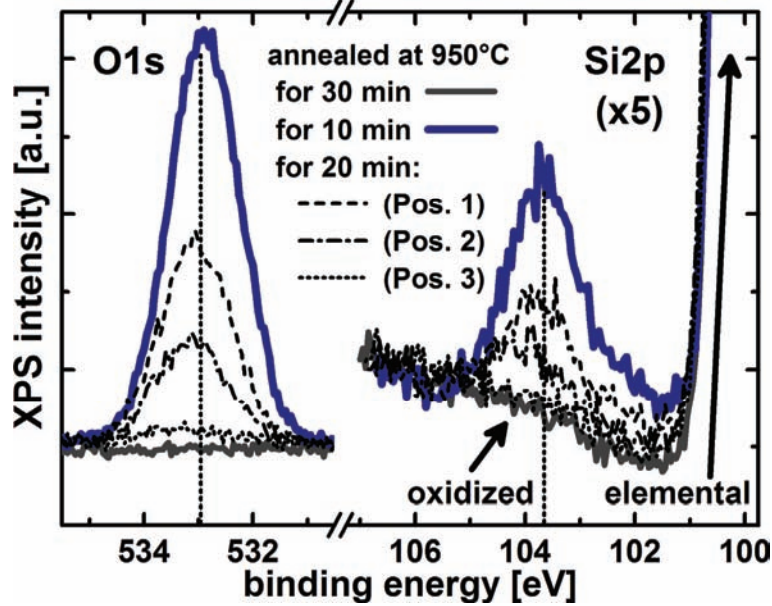
Figure 7: O1s and Si2p XPS lines measured at Si(100) substrates after annealing in the MOCVD reactor under pure H_2 flow at 950°C for 10 min (thick blue line), 20 min (broken black lines), and 30 min (grey line), respectively. The Si2p signal was amplified by a factor of 5 for better visibility of the oxidized share, while the main elemental line due to the substrate exceeds the applied scaling. The three broken black lines reflect very different residual oxide quantities coexistent on a single Si(100) substrate after the 20 min process at different, laterally distributed measurement positions.
