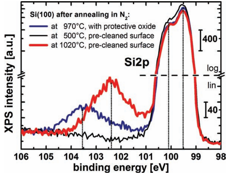
Figure 12: Si2p photoemission at an partially logarithmic intensity scale measured at the three Si(100) substrates also shown in Figure 11: Prior to annealing at surface temperatures of about 500°C (thin black) and 1020°C (thick red) in nitrogen at a pressure of 950 mbar, both samples were cleaned in hydrogen, while the third one was directly annealed in N 2 at 970°C (blue).
