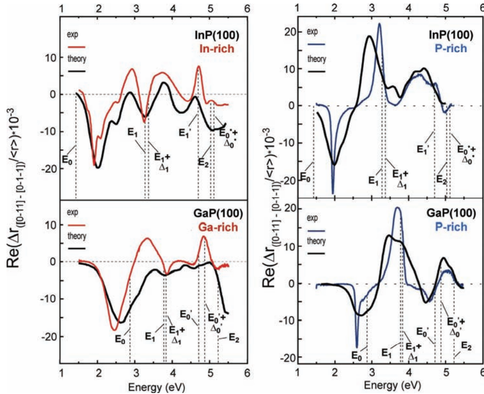
Figure 32: Comparison of theoretical RA spectra for III-rich [148] and P-rich [21,136] surfaces of InP(100) and GaP(100) to experimental data obtained at 20K [14].
