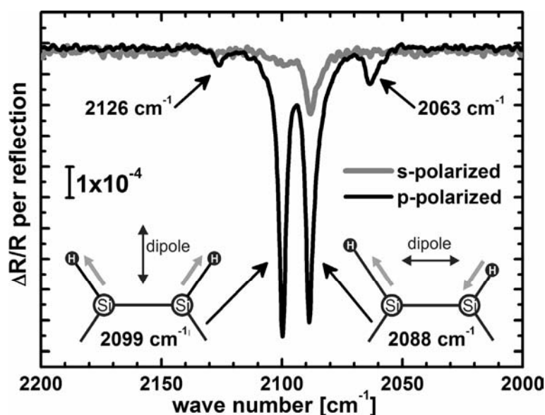
Figure 24: ATR-spectra of nearly single-domain Si(100) prepared by VPE employing s-polarized and p-polarized radiation: Absorption at 2099 cm -1 and 2088 cm -1 is assigned to the symmetric and antisymmetric stretch modes of the Si-H monohydride, respectively. The different intensity of the antisymmetric stretch mode in both s- and p-polarized spectra indicates a nearly single-domain Si(100) surface. Minor absorption lines at 2099 cm -1 and 2088 cm -1 are probably due to hydrogen bonds at double-layer step edges.
