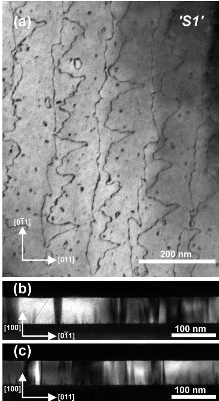
Figure 69: Structural characterization of the sample ‘S1’ by DF TEM: The imaging conditions for the plan-view (a) were chosen to visualize the APBs as dark lines, while the two different GaP phases show up with dark/bright contrast in the [0\bar{1}1] (b) and [011] (c) cross sections, respectively.
