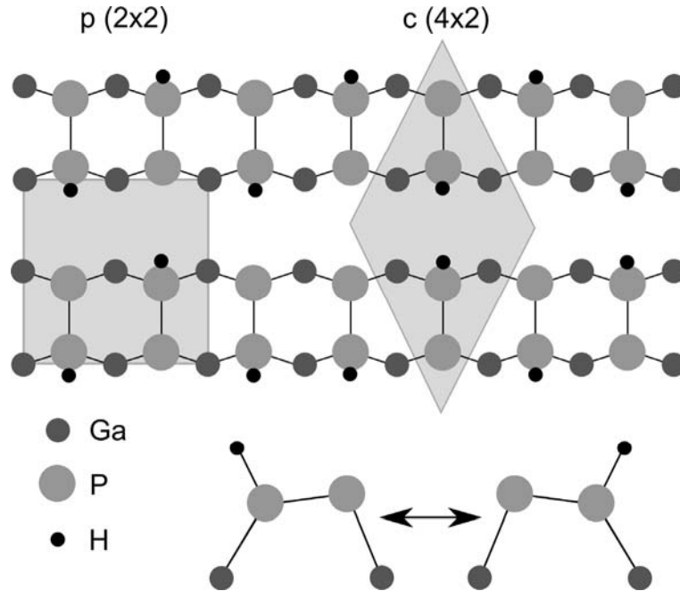
Figure 31: Top view and side view of hydrogen stabilized GaP(100) and InP(100) surface structure after Hahn et al. [21] and Schmidt et al. [136]. The unit cells are indicated in the top view.
