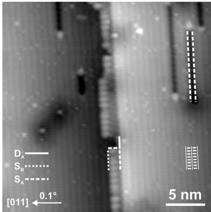
Figure 28: Atomic resolution empty state image of pseudo- D_A type step on a 0.1^\circ misoriented Si(100) surface. In most parts, the step consists of an S_A step and an S_B step, where the intermediate terrace is only a few dimers wide. On the terraces, vacancy islands consisting of missing dimer rows are visible ( V_{\text{sample}} = 760 mV, I_t = 840 pA).
