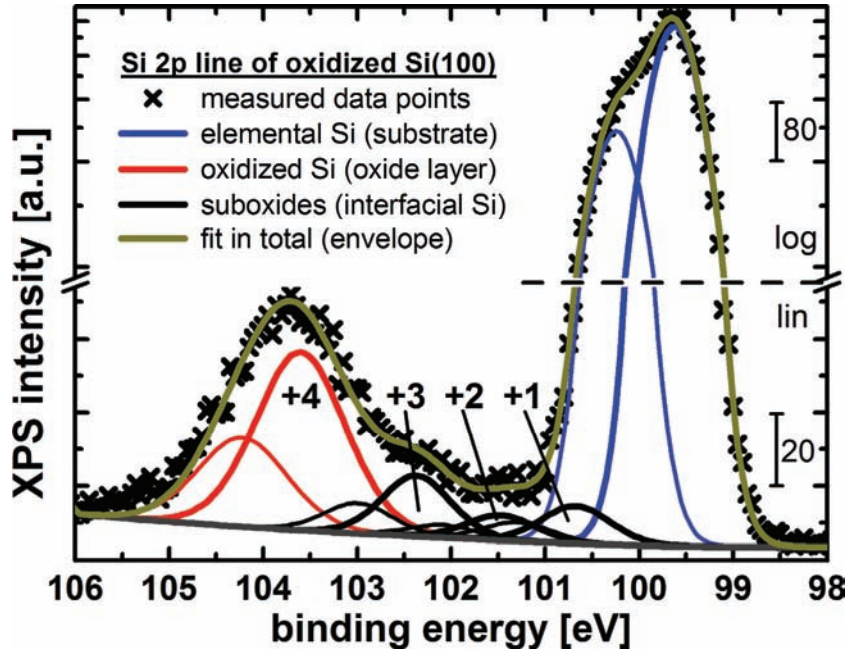
Figure 10: Deconvolution analysis of the Si2p XPS signal of a Si(100) surface that is still oxidized after annealing at 900°C in H 2 . Measurement with a photoelectron take-off angle of 30° provided enhanced surface sensitivity.
