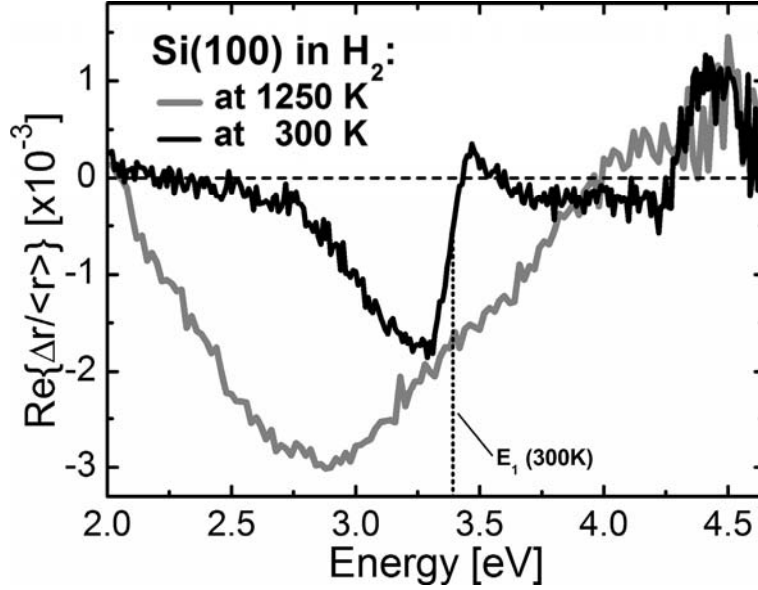
Figure 26: In situ RAS spectra of VPE-prepared Si(100), 6^\circ off-oriented in [011]: directly after deoxidation at 1250 K in hydrogen, the surface clearly shows the well-known, wide feature of a pure substrate, while the in situ signal after cooling to 300 K in the same ambient confirms a monohydride termination of the surface.
