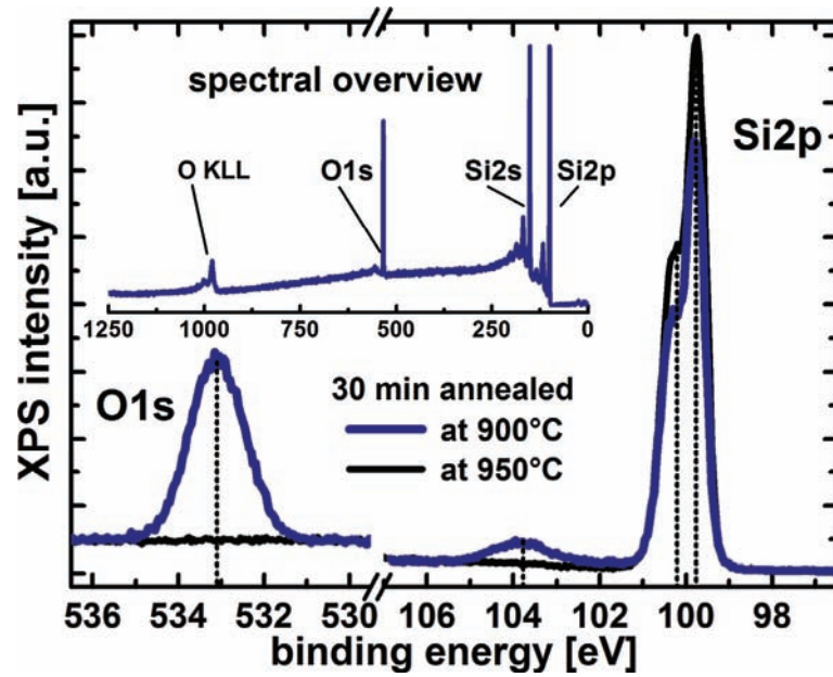
Figure 6: O1s and Si2p XPS lines measured at two Si(100) samples after annealing in the MOCVD reactor under pure H 2 flow for 30 min at 900°C (blue, thick) and at 950°C (black, thin) surface temperature, respectively and an XPS overview of the non-deoxidized sample (inset).
