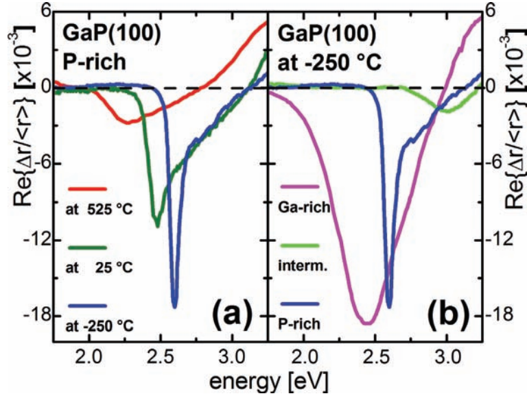
Figure 35: Low energy RAS peak of (a) the atomically ordered, P-rich, (2x2)/c(4x2) GaP(100) surface reconstruction at different temperatures and (b) of the P-rich and of the Ga-rich reconstructions as well as of the intermediate GaP(100) surface, all measured at the cryogenic temperature of -250 °C for higher spectral resolution.
