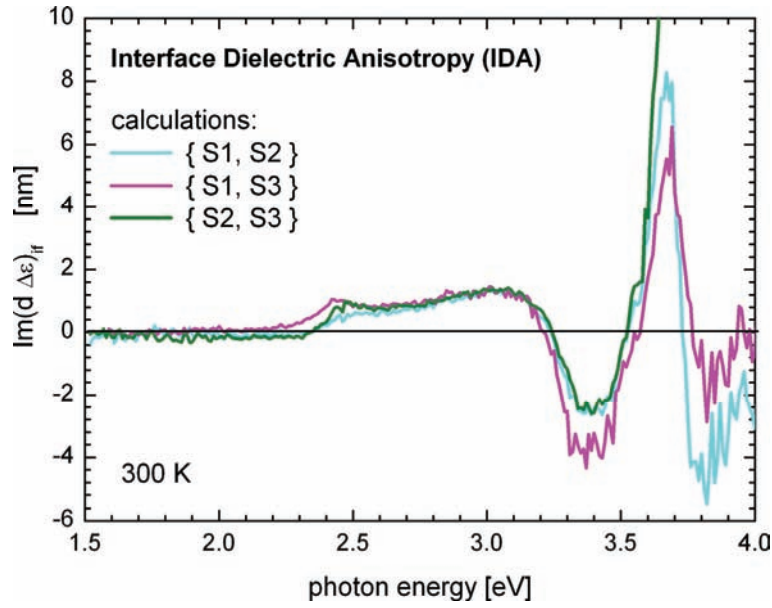
Figure 79: Calculated interface dielectric anisotropy (IDA) of GaP/Si(100) simultaneously derived by calculation of the SDA data shown in Figure 78. Due to excessive noise in the IDAs caused by absorption above the critical point energy of GaP at about 3.7 eV, the data is only shown up to 4.0 eV and one spectrum (green) had to be cut even earlier.
