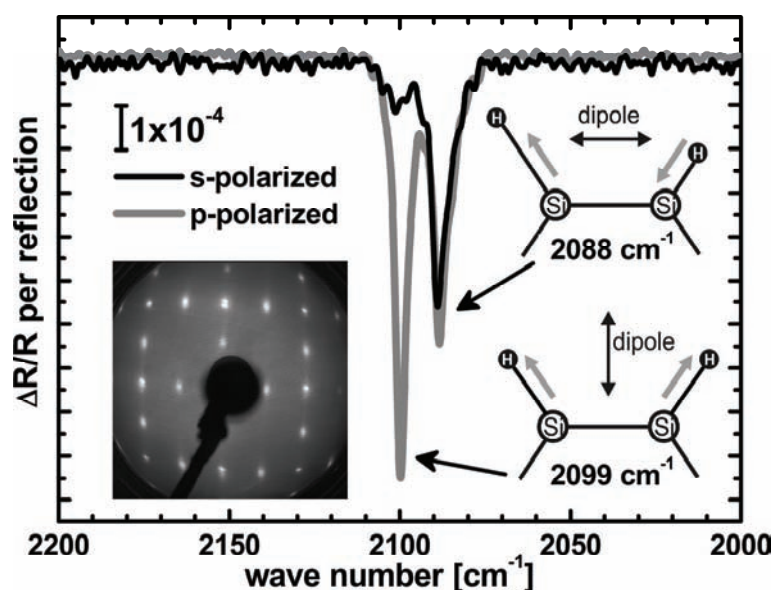
Figure 23: ATR-spectra of VPE-prepared Si(100) employing s-polarized and p-polarized radiation and associated LEED pattern (inset) of the same sample: Absorption at 2099 \text{cm}^{-1} and 2088 \text{cm}^{-1} is assigned to the symmetric and antisymmetric stretch modes of the Si-H monohydride, respectively. In agreement with the (2x1)/(1x2) symmetry observed by LEED, almost equal intensity of the antisymmetric stretch mode in both s- and p-polarized spectra indicates a two-domain Si(100) surface.
