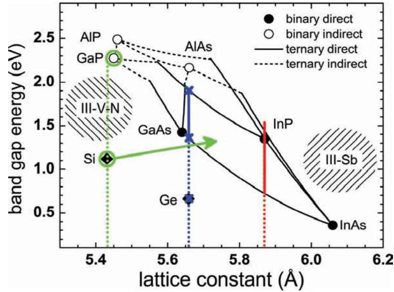
Figure 2: Band gap energies of classical elemental and III-V compound semiconductors over lattice constants. Solid and dashed black lines indicate ternary III-V materials, the enclosed area is available as quarternary or higher order compounds. Admixture of antimony and nitrogen may extend the range of material combinations significantly. Lattice matched heterostructures such as multi-junction solar cells can be grown on gallium arsenide, germanium (marked blue) and InP (marked red), while heterostructures on silicon (marked green) either involve significant lattice mismatch or the application of dilute nitrides.
