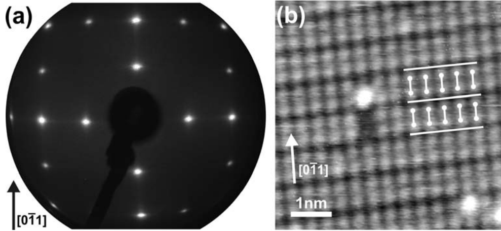
Figure 8: (a) LEED image of a deoxidized Si(100) surface at an incident beam energy of 70 eV exhibiting half-order reflexes due to a two-domain (2\times 1)/(1\times 2) reconstruction. (b) Empty state STM image of a deoxidized Si(100) surface ( V_{\text{Sample}} = 1.3 V, no filtering applied). Rows of individual dimers, which constitute a (2\times 1) surface unit cell, are clearly resolved.
