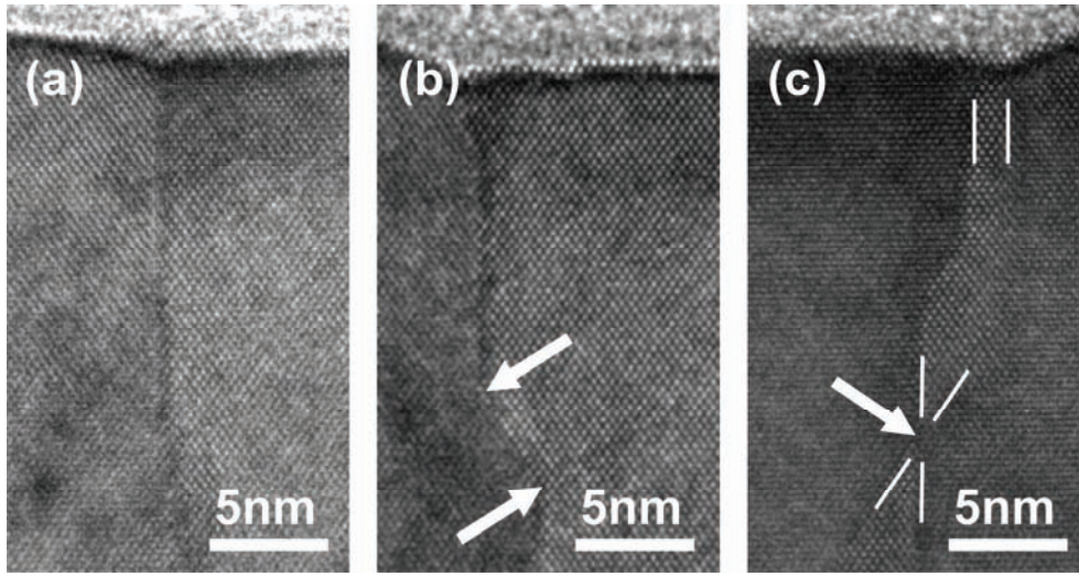
Figure 47: High-resolution TEM images displaying APBs obtained at cross-section specimens prepared from MOVPE-grown GaP films on Si(100) substrates with 0.1 misorientation. In general, APBs propagate in growth direction (a), but do not necessarily grow exactly straight (b). APB configurations which are not perpendicular to the image plane can appear twice (c).
