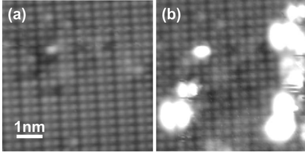
Figure 25: Empty states STM images (sample bias +1.2V) of MOVPE-prepared Si(100) before (a) and after (b) tip-induced hydrogen desorption: bright double-lobed features outshining the regular surface structure are indicative for pairs of dangling bonds.
