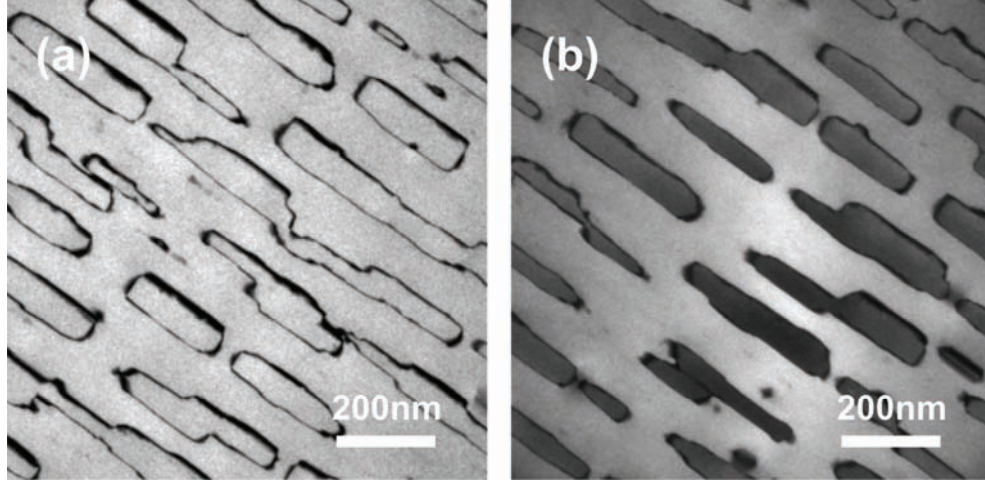
Figure 49: Plan-view TEM images with specific dark-field contrast for visualization of anti-phase disorder. Depending on the applied imaging conditions, either APBs appear with dark contrast (a) or dark/bright contrast between APDs and the main phase may be achieved (b).
