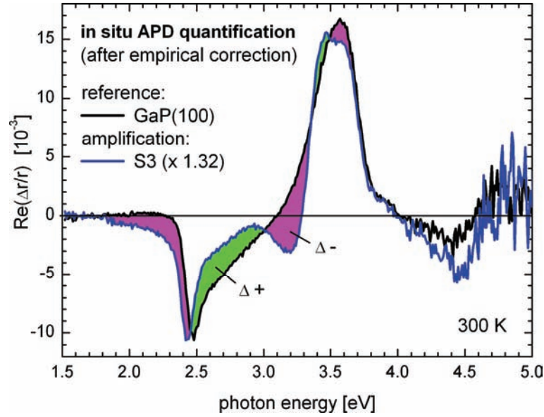
Figure 75: Empirical in situ RAS APD quantification applied to sample S3. After correction of the measured RA spectrum using the corresponding relative reflectance spectrum (Figure 74), empirical amplification of the intensity (blue) to match the intensity of the GaP(100) reference (black) estimates the APD concentration of the sample. Residual deviations of the sample spectrum (violet and green) potentially indicate optical anisotropy of the GaP/Si(100) heterointerface.
