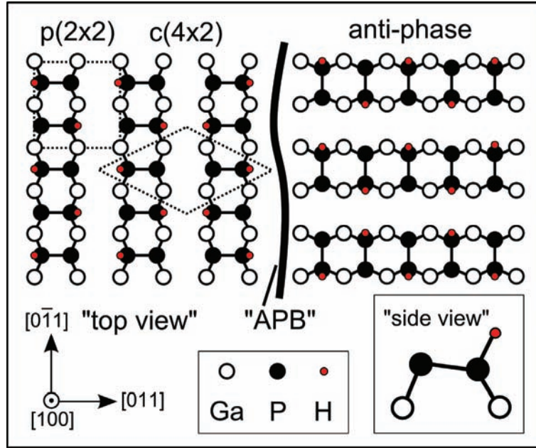
Figure 50: Dimer model of the P-rich GaP(100) surface reconstruction: Based on buckled P-dimers stabilized by a single hydrogen atom (see inset), the surface is arranged in parallel and anti-parallel dimer rows resulting in a combined p(2 \times 2)/c(4 \times 2) symmetry (left). Only on hetero-epitaxial GaP/Si(100) surfaces, also perpendicular dimer orientation occurs (right) due to anti-phase disorder.
