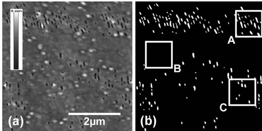
Figure 60: AFM characterization of the GaP/Si(100) surface after specific annealing: The AFM image (a) identifies APDs by induced height contrast. The transfer to color-coded image (b) highlights the APD content determined to be 3.1%. The marked regions are discussed in the main text.
