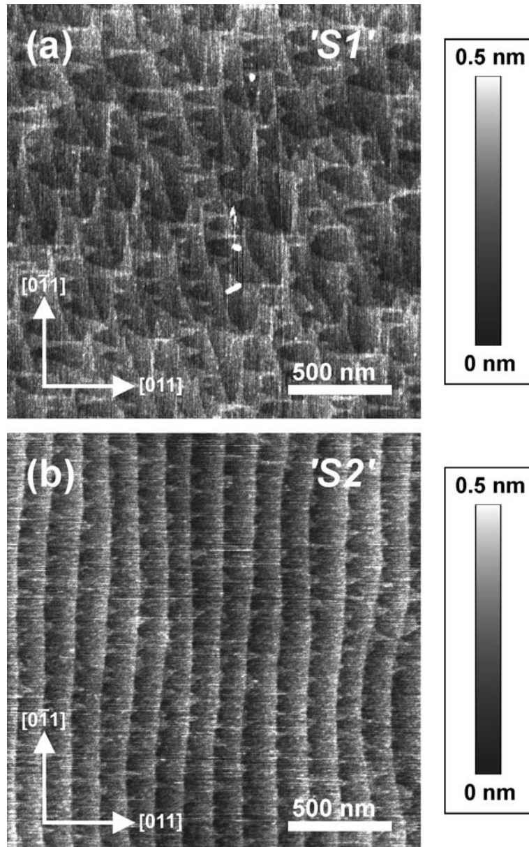
Figure 65: Ex situ AFM characterization of Si(100) surfaces after identical VPE preparation processes applied to about 0.1^\circ misoriented substrates with projection of the off-cut pointing either about 30^\circ off from (type 'S1') and almost exactly in (type 'S2') the [011] direction, respectively: While the first configuration (a) led a two-domain surface with complex structure, but without a clearly recognizable preference, the latter (b) enabled a significant predominance of the surface area covered by one domain orientation compared to the other one.
