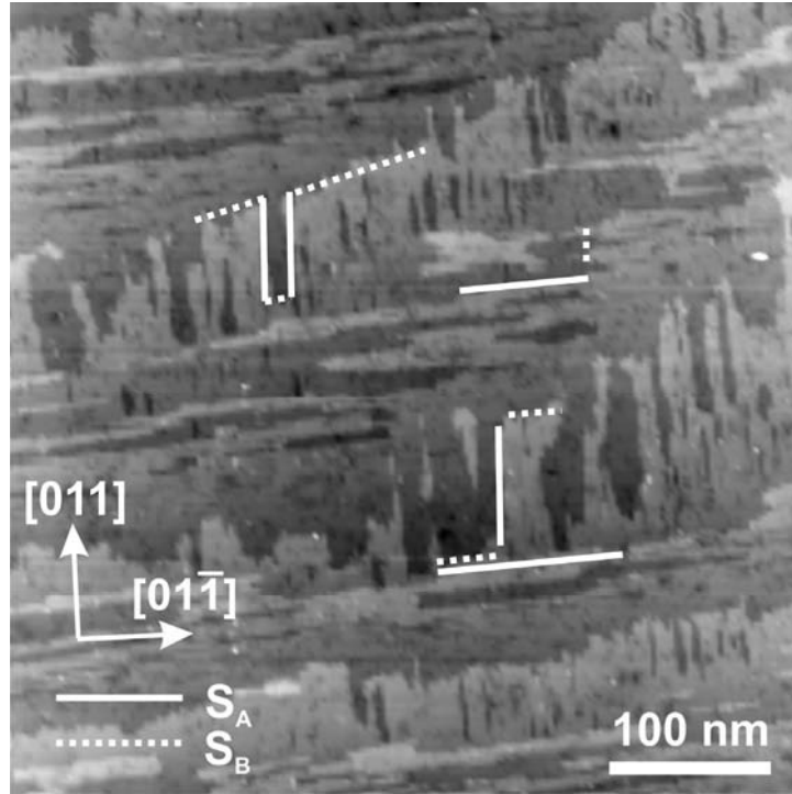
Figure 16: Empty state image ( V_{\text{Sample}} = +1.2 V, I_t = 400 pA) of a thermally deoxidized Si(100) surface on a substrate with 0.1^\circ misorientation toward [011] : Frayed monolayer steps dominate the surface structure, the alternating directionality allows straightforward differentiation between S_A and S_B type steps.
