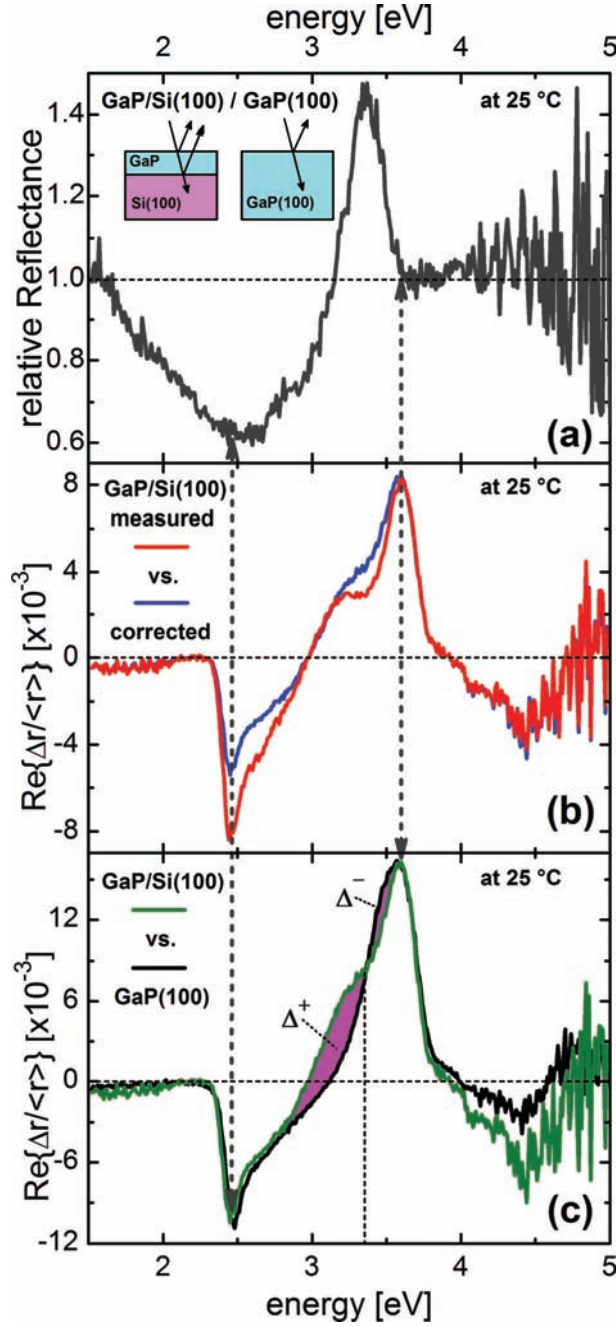
Figure 59: Measurement of an about 30 nm thin GaP film deposited on a Si(100) substrate in comparison to a homoepitaxially grown GaP(100) sample, all conducted at room temperature (25 °C). (a) Relative reflectance R_{\text{rel}}^{\text{spl}}(\lambda) (see text) that was used for correction of the Fabry-Pérot oscillations in the measured data of the heteroepitaxial sample reflection. (b) Comparison of the originally measured RA spectrum (curve with highest peak at 2.5 eV) and the corrected RA spectrum (curve with smaller peak) according to equation 10. (c) Comparison of the corrected RA spectrum that was scaled up by a factor of m = 1.94 to fit the reference RA spectrum taken from an APD free homoepitaxially GaP(100) sample.
