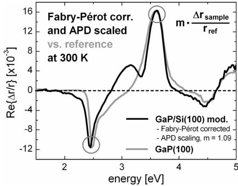
Figure 64: Complete correction of the RA spectrum from the heteroepitaxial GaP/Si(100) sample shown in Figure 61. The convolution of the relative reflectance to the measured RA spectrum corrected the interference influence on the normalization. Afterwards, linear scaling of the calculated spectrum compensated signal reduction caused by APDs. The peaks intensities now match more accurately.
