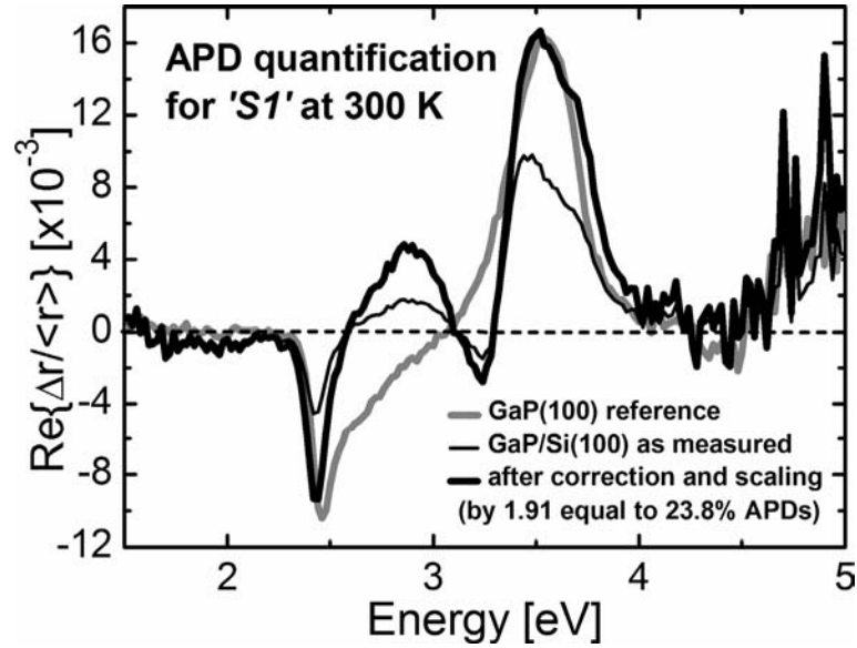
Figure 67: Quantitative in situ RAS analysis of the anti-phase disorder in the GaP/Si(100) film grown on the distinctly two-domain substrate ‘S1’: The measured data (thin black curve) required the correction of interferences via the relative reflectance prior to linear scaling of the signal (thick black curve) to the intensity of the homoepitaxial reference signal (thick grey curve) eventually resulted in the determination of APD concentration of the sample of about 23.8%.
