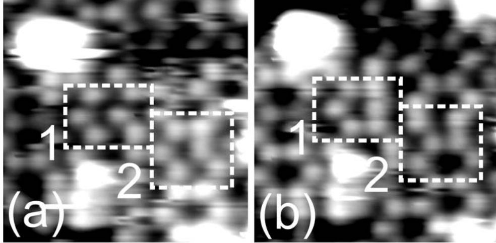
Figure 43: Consecutive filled state images of GaP(100) surface at room temperature. Frames 1 and 2 indicate regions where dimer flipping occurs between the images. The time elapsed between images is about 1 minute, while the time required to completely image one atom is about 1.5 s. Scale 45 \text{ \AA} \times 45 \text{ \AA} .
