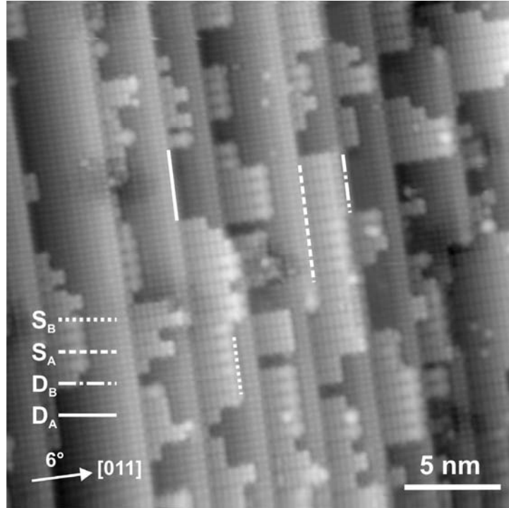
Figure 30: Atomic resolution empty state image of 6° misoriented Si(100) surface. The step structure consists of a mixture of S_A , S_B , D_A and D_B type steps, with no clear preference for one of the step types. ( V_{\text{sample}} = 1240 mV, I_t = 190 pA).
