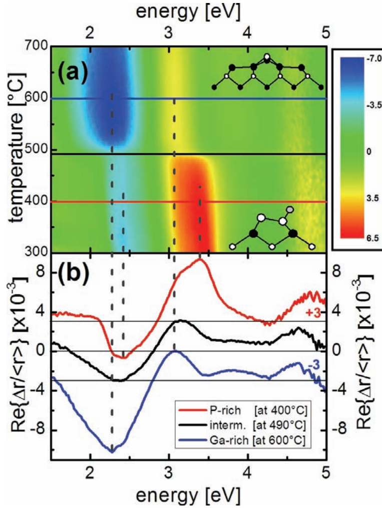
Figure 56: (a) In situ RAS colorplot of the surface of a heteroepitaxial GaP film which was grown on 2° off-orientated Si(100): In direct analogy to Figure 33, spectra were taken continuously while the sample temperature was ramped up from 300 to 700°C at a rate of 1.5 K/min without TBP supply. Qualitatively, we observed the P-rich surface reconstruction between 300°C and 490°C, the Ga-rich reconstruction beyond 500° C and an intermediate surface state in a narrow range around 490 °C – 500 °C as expected in analogy to homoepitaxial GaP(100). (b) Extracted RA spectra which represent the P-rich (top), the Ga-rich (bottom) and the intermediate surface (middle). Dashed vertical lines connect the peak positions with the respective features in the colorplot.
