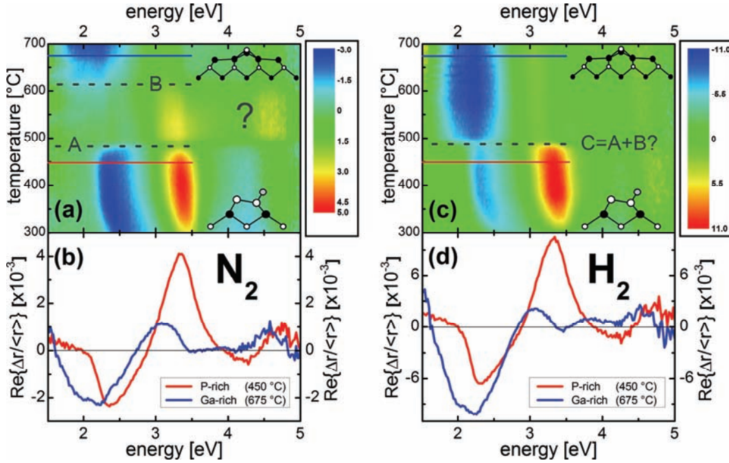
Figure 37: Comparison of the MOVPE-preparation of GaP(100) surfaces in nitrogen (a, b) and hydrogen (c, d) by means of color-coded in situ RAS results (a, c) measured while the sample temperature was ramped up slowly (at a rate of 1.5 K/min) from 300°C to 700°C without TBP supply.
