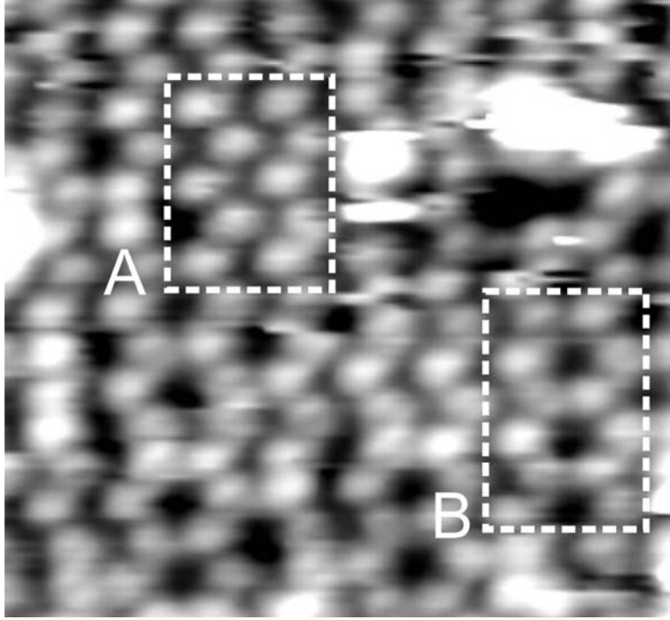
Figure 42: Filled state image of GaP(100) surface at room temperature. Regions A and B exhibit p(2 \times 2) and c(4 \times 2) reconstructions, respectively. Scale 65 \text{ \AA} \times 60 \text{ \AA} .
