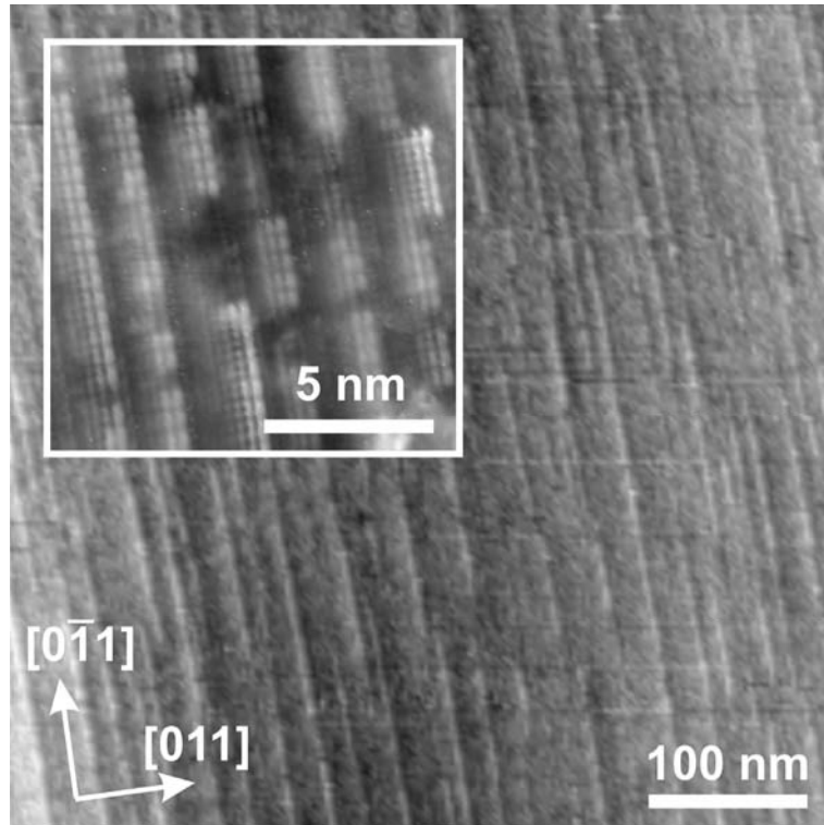
Figure 20: Empty state images of thermally deoxidized Si(100) with 6^\circ misorientation in [011] direction: The large scale image ( V_{\text{Sample}} = +1.3\ \text{V} , I_t = 70\ \text{pA} ) shows step structures with irregular spacing, while the inset ( V_{\text{Sample}} = +0.9\ \text{V} , I_t = 520\ \text{pA} ) depicts a region with predominantly double layer steps in high-resolution where the Si dimers are clearly visible.
