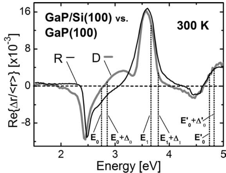
Figure 53: Comparison of the RA spectra of sample D and of a homoepitaxially prepared GaP(100) reference R .
