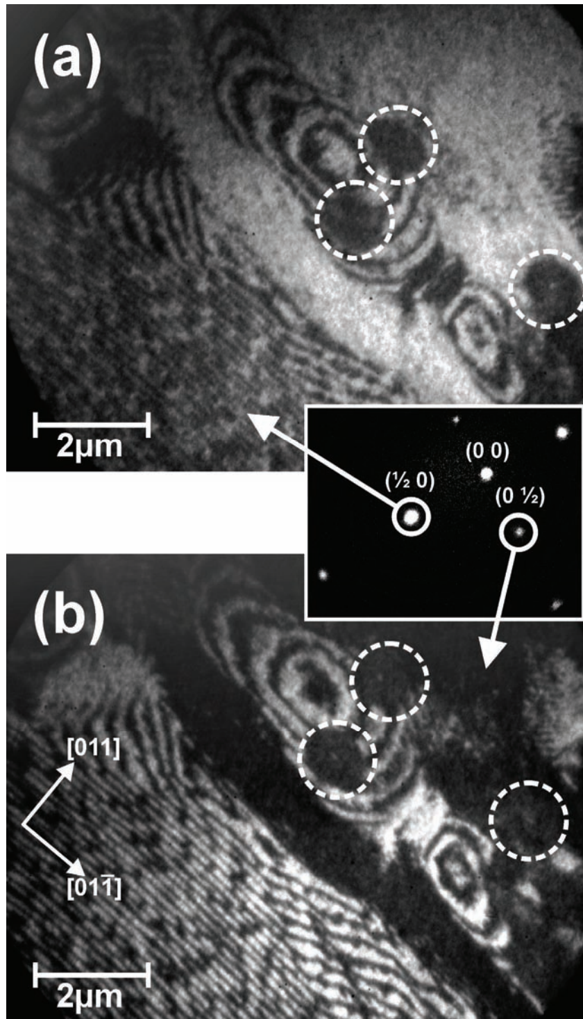
Figure 71: Phase-selective LEEM images ( E_p = 10.2\text{eV} ) of anti-phase disorder in a heteroepitaxial GaP/Si(100) film: dark-field imaging with the characteristic (\frac{1}{2} 0) (a) and (0 \frac{1}{2}) (b) diffraction reflexes (see inset for LEED pattern at E_p = 9.7\text{eV} ) results in high contrast of the respective domain orientations. Encircled spots can not be attributed to neither of the phases.
