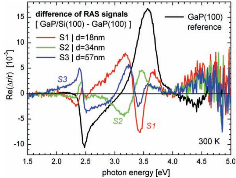
Figure 76: Deviation of the GaP/Si(100) RAS spectra shown in Figure 73 from the GaP(100) reference spectrum (black) after full empirical correction.
