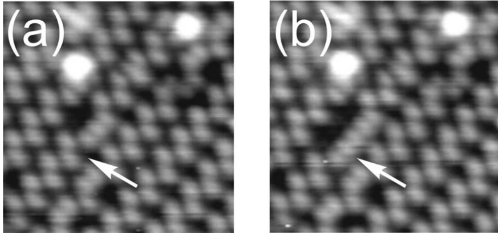
Figure 45: STM observation of a dimer-flipping process at a InP(100) p(2 \times 2)/c(4 \times 2) surface unit (indicated by arrows) in two successive occupied states STM images measured at room temperature. Such flipping processes have been observed several times at different locations on the surface. Scale 58 \text{ \AA} \times 58 \text{ \AA} , sample bias voltage: -5.2 \text{ V} .
