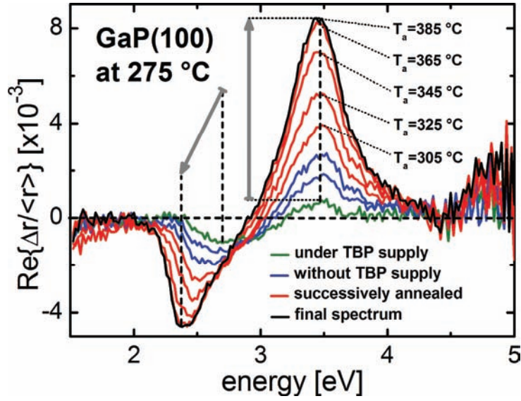
Figure 36: RAS spectra of a GaP(100) sample, all taken at 275 °C, when successively preparing the atomically ordered (2x2)/c(4x2) surface reconstruction. The first spectrum was taken with TBP supply (lowest intensity), followed by two successive spectra just without TBP supply (increasing intensities). Then, the sample was annealed for short times at successively increasing temperatures and cooled down to 275 °C for the measurement of the individual RA spectra ( T_a > 300^\circ\text{C} ) until reaching the final RA spectrum of the P-rich surface (highest intensity).
