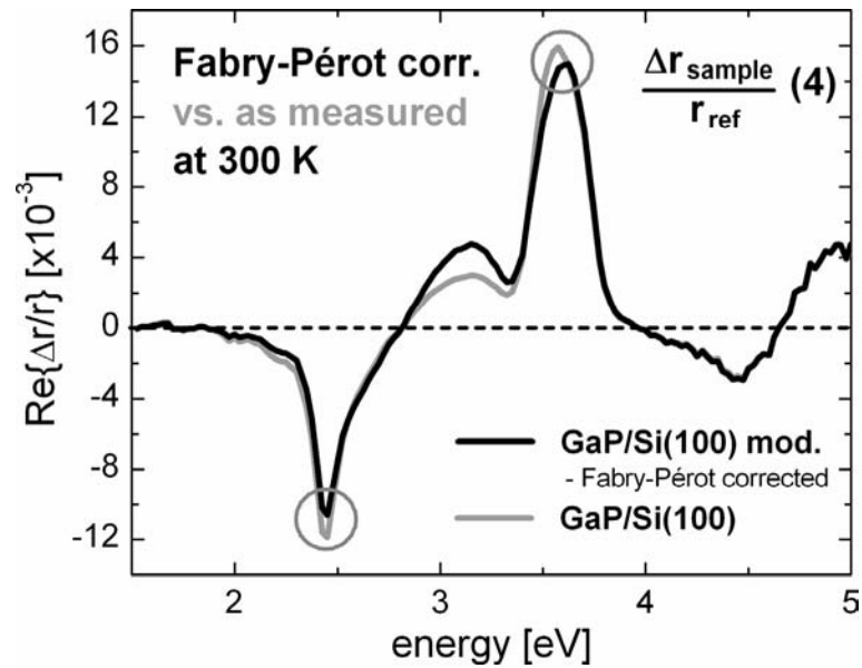
Figure 63: Comparison of the measured RA spectrum from the heteroepitaxial GaP/Si(100) sample shown in Figure 61 with the “artificial” spectrum (see text) according to Eq. 10, i.e. the convolution of the measured spectrum with the relative reflectance. Both peaks slightly decrease in intensity, the negative peak more than the positive one.
