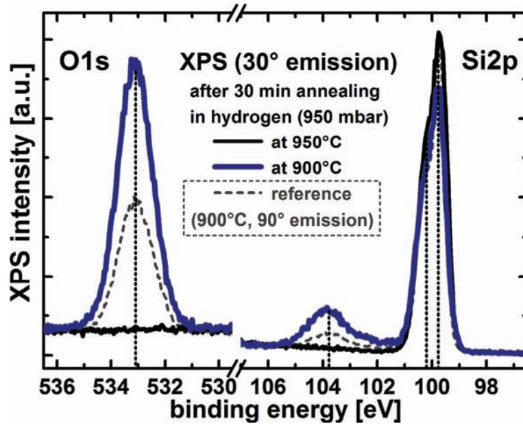
Figure 9: O1s and Si2p XPS lines measured under a photoelectron take-off angle of 30° at two Si(100) samples after annealing in a MOVPE reactor under pure H 2 flow for 30 min at 950°C (black, thin) and at 900°C (blue, thick) surface temperature, respectively. The comparison with normalized XPS data of the sample prepared at 900°C measured under normal photoemission (grey, thin) confirmed the expected gain of surface sensitivity.
