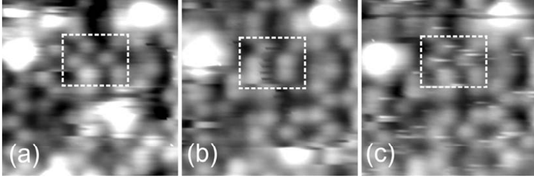
Figure 44: Consecutive filled state images of GaP(100) surface at 120 K. The frame indicates a location where two dimers flip back and forth in the images. The time elapsed between consecutive images here is about 16 s, while the time required to completely image one atom is about 0.4 s. Scale 45 \text{ \AA} \times 45 \text{ \AA} .
