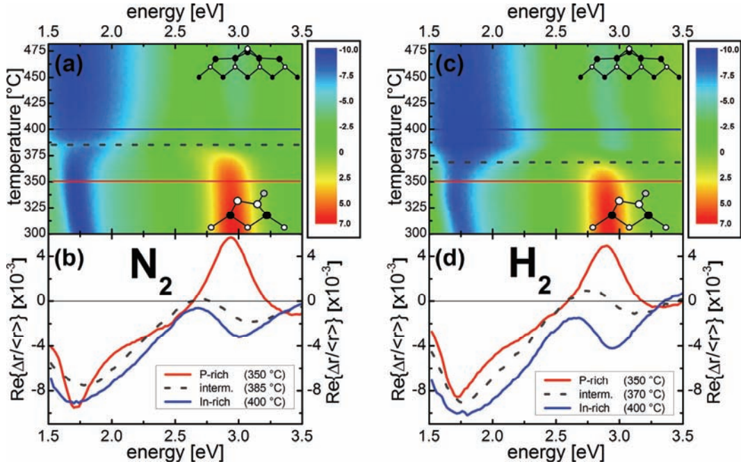
Figure 40: Comparison of the MOVPE-preparation of InP(100) surfaces in nitrogen (a, b) and hydrogen (c, d) by means of color-coded in situ RAS results (a, c) measured while the sample temperature was ramped up slowly from 300°C to 480°C without TBP supply.
