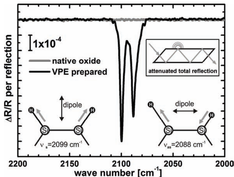
Figure 22: Surface sensitive FTIR spectra measured in an attenuated total reflection (ATR) configuration at a \text{Si}(100) sample before (grey) and after (black) thermal oxide removal in H_2 . Clear features emerged in the region around 2100\text{ cm}^{-1} and can be assigned to the symmetric and asymmetric stretch modes of coupled Si-monohydrides.
