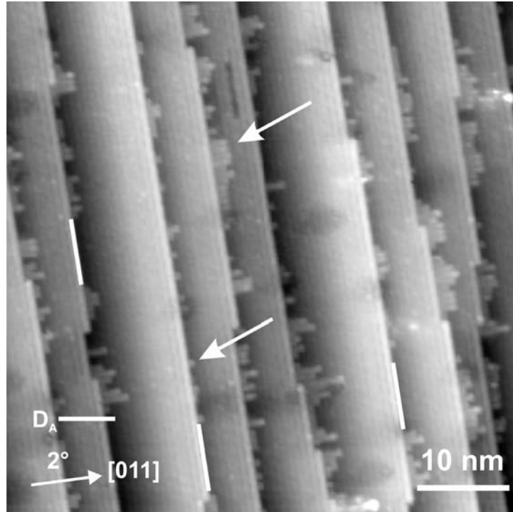
Figure 29: High resolution empty state image of step structure on a 2^\circ misoriented Si(100) surface consisting largely of D_A type steps. In some parts, residuals of the intermediate terrace, consisting of dimer rows of varying length, extend from the A-type step onto the terraces ( V_{\text{sample}} = 1240 mV, I_t = 190 pA).
