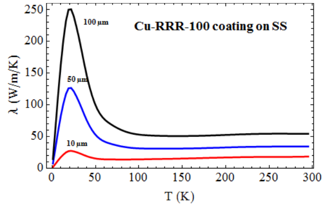
Figure 3: Thermal conductivity.
