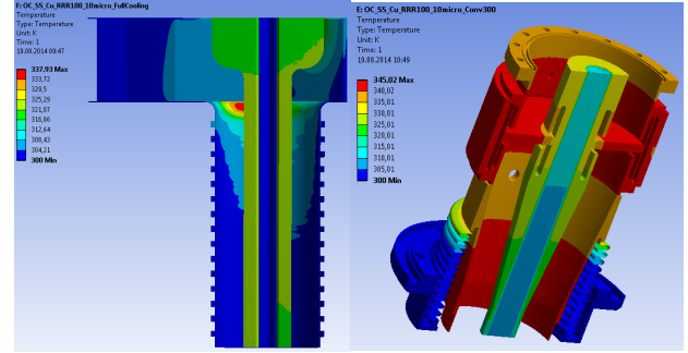
Figure 5: Thermal simulation: in case of no reflection.
