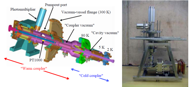
Figure 1: The TTF III coupler (left) and test stand (right).
