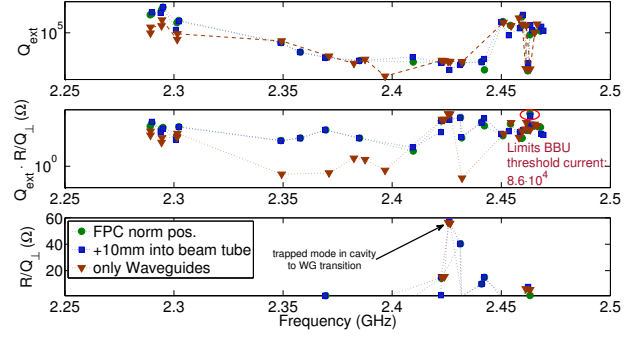
Figure 3: Comparison of Q_{\text{ext}} , R/Q_{\perp} and the BBU parameter R/Q_{\perp} \cdot Q_{\text{ext}} for the TTF FPC at nominal position (green dots), 10 mm more into the beam tube (blue squares) and a symmetric system with six waveguides.
