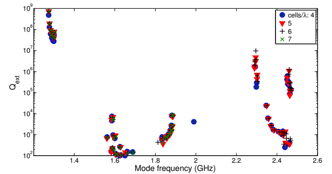
Figure 5: Convergence study of Q_{\text{ext}} for the HOM spectrum using different mesh densities with the hexahedral mesh of CST 2014 using eight cells per max model box edge .
