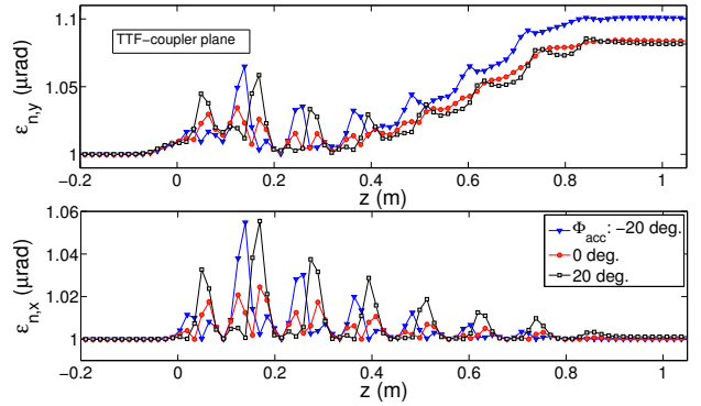
Figure 8: Emittance evolution in both transverse planes for the bERLinPro design.
