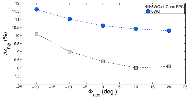
Figure 6: Relative emittance growth in the vertical planes versus \phi_{\text{acc}} for the 5WG+coax FPC structure and the 6WG cavity in reference to the bare cavity using the PIC code.
