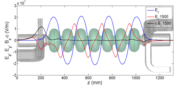
Figure 7: On-axis longitudinal and transverse field components for an electric wall boundary condition for the standing wave regime.
