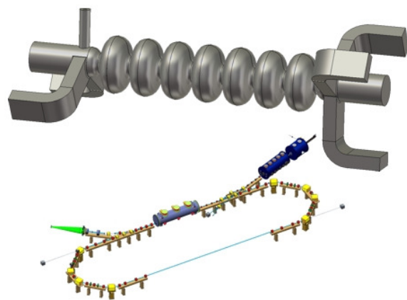
Figure 1: Scheme of the bERLinPro ERL with the main linac section within the recirculating ring. Above the linac cavity structure is shown including the FPC and five waveguides for HOM damping.
