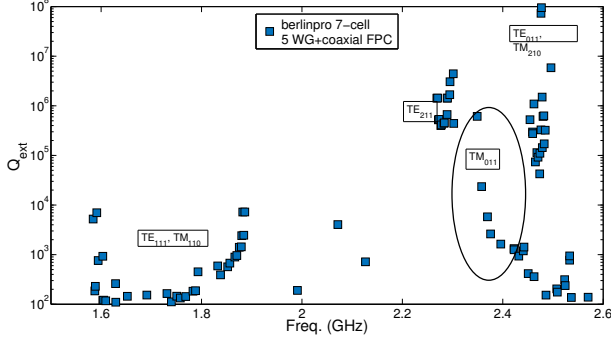
Figure 2: External Q for the 7-cell bERLinPro linac cavity featuring one coaxial FPC and five waveguide based HOM absorbers obtained by CST MWS eigenmode computations.
