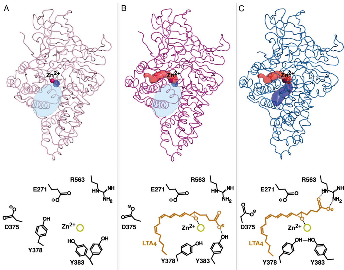
Fig. 4. Tunnel formations (Upper; the structures and corresponding \text{Zn}^{2+} are colored as in Fig. 3 B and C) and proposed mechanism of substrate binding (Lower) during dynamic domain motion between open and closed D375N. (A) In the open conformation (polar part of binding pocket is shown as tiny blue spot; wide space between domains at the entrance of the active site is indicated as an oval in shaded light blue) Y378 blocks the entrance of the hydrophobic cavity. (B) During substrate binding, lid region moves and opens the hydrophobic tunnel (red surface representation) for \text{LTA}_4 entrance. When \text{LTA}_4 slides into the hydrophobic pocket, its carboxylate group is guided by Y383. (C) During domain motion, the \omega -end reaches the bottom of the cavity, the epoxide binds to \text{Zn}^{2+} , and the C1 carboxylate switches from Y383 to R563. The closed conformation affords productive substrate alignment and allows epoxide activation and subsequent hydrolysis according to an \text{S}_{\text{N}}1 mechanism. The polar arm of the binding pocket that is formed as a result of convergence of domains is shown as blue surface.
