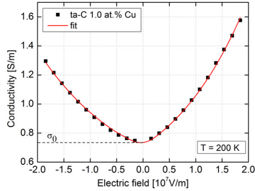
Figure 5. Conductivity of ion tracks in ta-C (doped with 1 at.% Cu) at 200 K as a function of applied electrical field E = V/d . The sample was irradiated with 1 GeV U ions to a fluence of 4 \times 10^9 ions \text{cm}^{-2} . The solid line is a fit with the stretched exponential function and an asymmetry term (see section 3.4).
