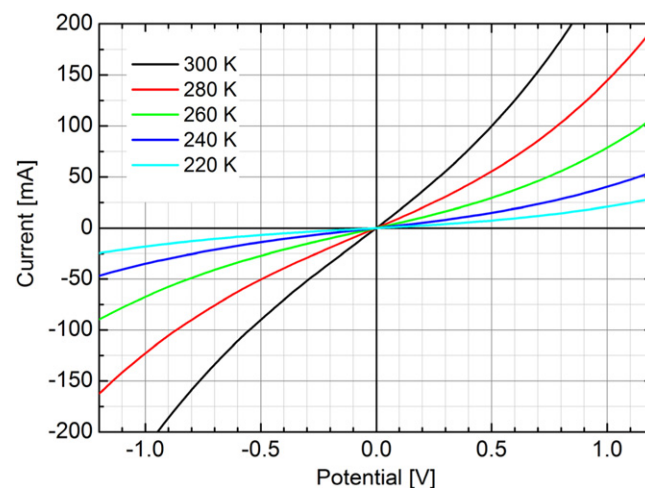
Figure 4. Current–voltage ( I – V ) characteristics measured with a macroscopic contact pad ( 0.6 \text{ mm } \varnothing , averaging over about 10^7 ion tracks) at different temperatures for the 1 at.% Cu-doped sample.
