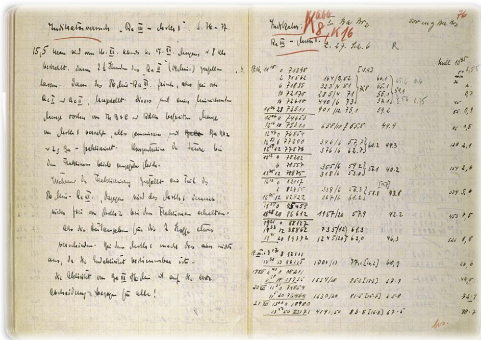
O. Hahn: Discovery of nuclear fission
