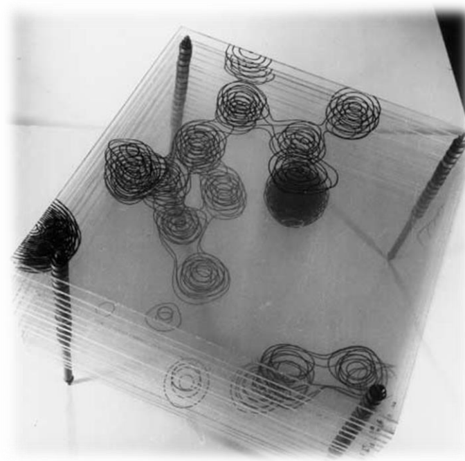
Dorothy Hodgkin's three-dimensional electron density model of penicillin
