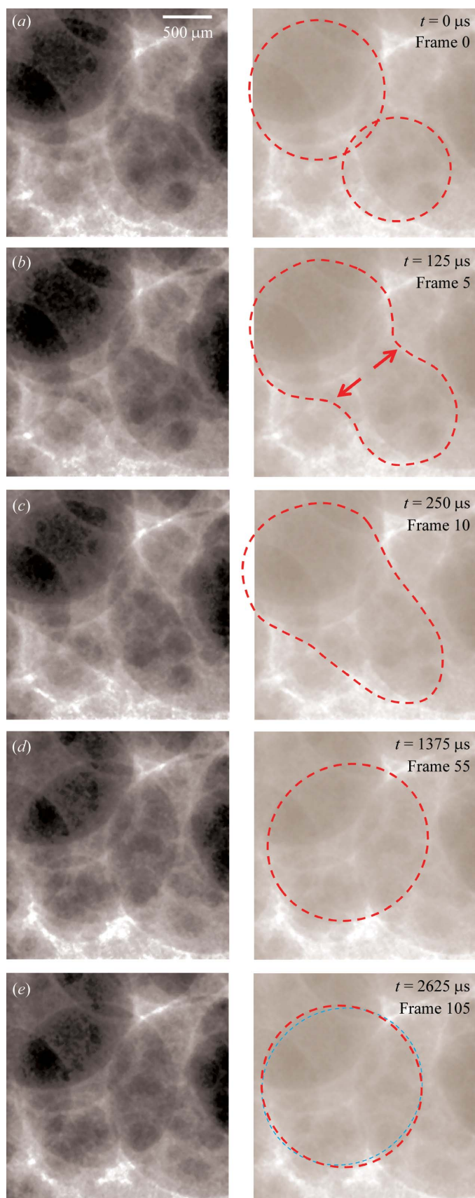
Figure 1 Left column: selected images of a series of 184000 showing film rupture in (a) to (c) and bubble oscillation in (d) and (e). Right column: features discussed in the text.
