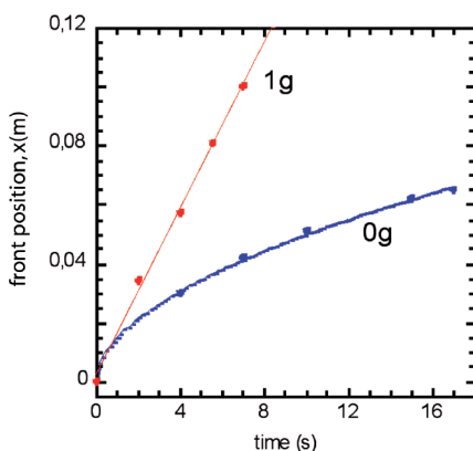
◀ FIG. 1: Position of the liquid front in forced drainage experiments: red circles, on ground, the liquid velocity is constant; blue circles, in 0g: the propagation is diffusive and slower, allowing one to reach much larger volume fractions – instabilities seen on ground are prevented [2].
