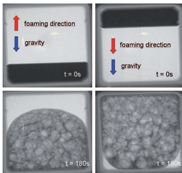
▲ FIG. 2: X-ray radiograph of ground tests of the aluminium foam furnace successfully used in the sounding rocket experiment of April 2008. Various configurations were tested, including foaming against gravity (left panel, "1g") and supported by gravity (right panel, "-1g") and tests were also performed on parabolic flights. All flight data are being analysed.
