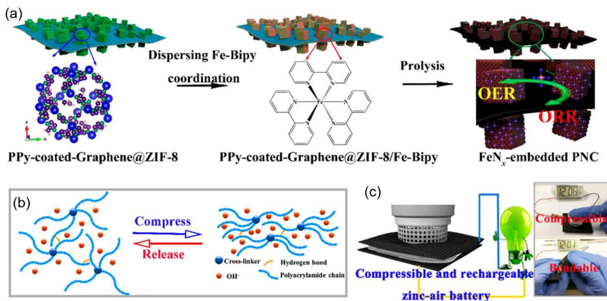
Figure 33. (a) Synthesis of Fe x N embedded in 2D porous nitrogen-doped carbon. Local amplification shows the structure of ZIF-8, coordination of (iron ion)-(2,2-Bipy), and Fe x N dispersed on the porous nitrogen-doped carbon surface. (b) Compressible polyacrylamide hydrogel, and (c) compressible, bendable, rechargeable zinc–air battery. Reproduced with permission from ref 485. Copyright 2018 American Chemical Society.
