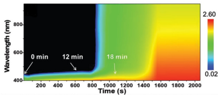
Figure 3. The time-resolved absorption spectrum of a blade-coated PVK film under natural drying, demonstrating a processing window up to 12 mins [55]. John Wiley and Sons [55]. (Copyright © 2019 WILEY-VCH Verlag GmbH & Co. KGaA, Weinheim.)
