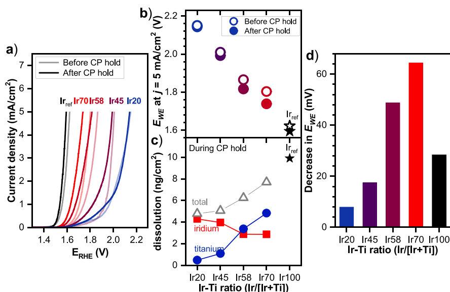
Figure 2. (a) Anodic polarization curves from 1.2 V_{RHE} to E_{WE} at j = 5 \text{ mA/cm}^2 recorded with a scan rate of 10 mV/s (EP step 2. and EP step 4. before and after CP hold) for samples Ir20, Ir45, Ir58, and Ir70 of the compositional Ir-TiO x material library. The reference measurement on a sputter deposited metallic Ir thin film ( Ir_{ref} = Ir100 ) used as an internal benchmark for an iridium concentration of 100% is shown in black. (b) OER activity represented by E_{WE} at j = 5 \text{ mA/cm}^2 during the LSVs for the compositional Ir-TiO x material library. The open circles correspond to LSVs before the CP hold (EP step 2.), and the filled circles correspond to LSVs after the CP hold (EP step 4.). The reference measurements on Ir_{ref} are shown in black stars. (c) OER stability obtained from the iridium and titanium dissolution quantities (and their totals = iridium + titanium) obtained during the CP hold at 1 \text{mA/cm}^2 for 2 min (EP step 3.) for the compositional Ir-TiO x material library. The reference measurements on Ir_{ref} are shown in black stars. (d) OER activity improvement shown as the change (decrease) in the E_{WE} at j = 5 \text{ mA/cm}^2 value after the CP hold at 1 \text{mA/cm}^2 for 2 min (EP step 3.) for the compositional Ir-TiO x material library. The reference measurement on Ir_{ref} is shown in black. All measurements were performed in 0.1 M HClO 4 .
