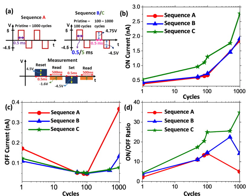
Figure 6. (a) Cycling and measurement sequences used for studying the impact of cycling pulses on the ON and OFF currents. Sequence A represents asymmetric cycling with +5 and −4.5 V with a pulse width of 0.5 ms from pristine to 1000 cycles. Sequence B corresponds to asymmetric cycling of +5 and −4.5 V with a pulse width of 0.5 ms from pristine to 100 cycles followed by asymmetric cycling of +4.75 and −4.5 V with a pulse width of 0.5 ms from 101 to 1000 cycles. Sequence C is similar to sequence B except for the pulse width of 5 ms during the first 100 cycles. Reset and set operations are performed with +4.5 and −4.5 V square pulses with a pulse width of 0.5 ms. The read operation of the OFF and ON states is performed with a DC bias of −1.6 V. (b, c) Evolution of the ON and OFF currents, respectively, from pristine to 1000 cycles for pulse sequences A, B, and C. (d) Evolution of the ON/OFF ratio from pristine to 1000 cycles for pulse sequences A, B, and C.
