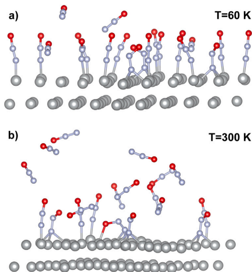
Fig. 7. Snapshots of N_2O monolayer on Ni(111) after 3 ps of the AIMD simulation at 60 K (top panel) and 300 K (bottom panel) within NVT thermostat and a time step of 1 fs.
