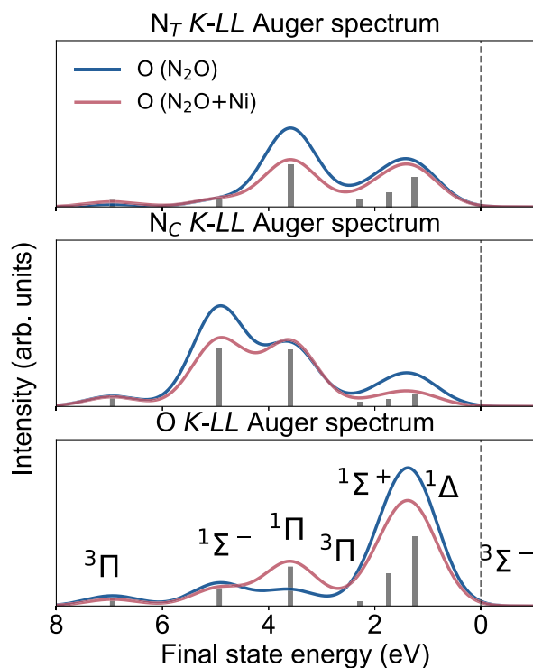
Fig. 4. Theoretical Auger spectrum obtained with the one-center approximation for both single N_2O and N_2O+Ni systems, calculated at the N_T K-edge (top), N_C K-edge (middle) and O K-edge (bottom). The energies in the horizontal axis are calculated using the ^3\Sigma^- state as the reference. The molecular symbols in the bottom plot are the same for the other graphics.
