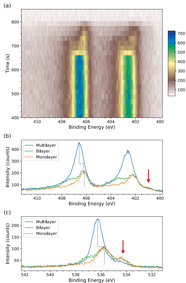
Fig. 1. (a) shows the evolution of the N 1s core level while heating the sample. At 650 s the thermocouple readout was 39 K and at 800 s 42 K with all molecules desorbed, further discussed in the text. The bottom two panels shows 3 typical spectra of N 1s (b) and O 1s (c) of multilayer, bilayer and monolayer coverage. With dashed lines highlighting the binding energy shifts of the different coverages and red arrows the binding energy of dissociated O and N.
