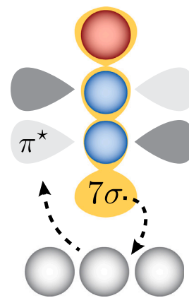
Fig. 9. Schematic view of the backdonation.
