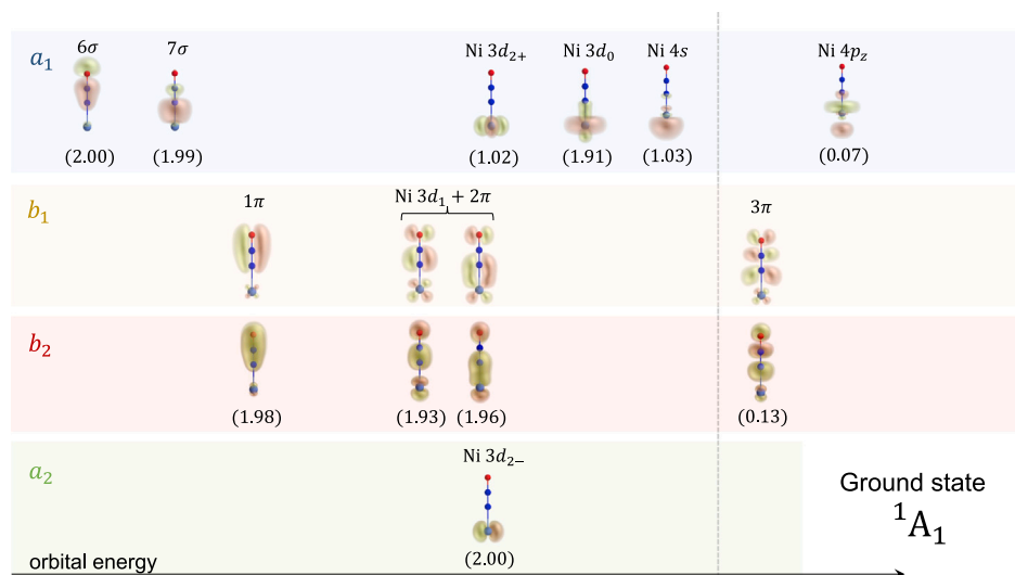
Fig. 3. Diagram of the active space used for describing the ground state of the N_2O+Ni idealized structure. The MOs are disposed according to the symmetry components of the C_{2v} point group, and they are arranged by orbital energy from left to right. The vertical dashed line divides the occupied orbitals (left) from the unoccupied orbitals (right). Numbers in parenthesis denote natural occupation numbers.
