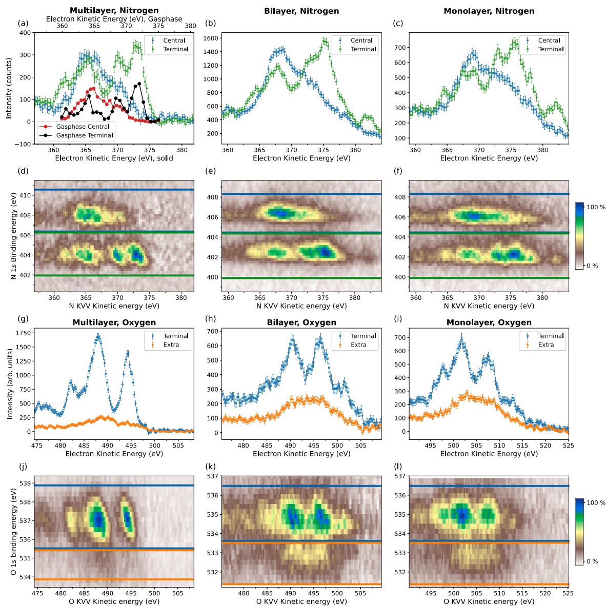
Fig. 2. Panels a–f show the N coincidence maps and integrated spectra from the regions marked with colored lines in the coincidences maps. Panel a also shows a comparison to the coincidence spectra from gas-phase N_2O , the gas-phase data is taken from Ref. [26], note the top energy axis for the gas-phase reference. Panels g–l shows the corresponding O coincidence data.
