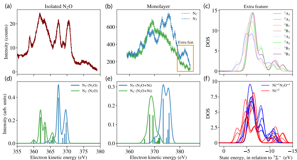
Fig. 5. (a) Experimental Auger spectrum for isolated \text{N}_2\text{O} , as a function of the electron kinetic energy, in eV, from Ref. [22]. (b) Experimental Auger spectrum for the monolayer, as a function of the electron kinetic energy, in eV. (c) Detailed composition of the extra structure at 380–385 eV in panel (b), showing density of doubly charge states with energies below {}^3\Sigma^- , colored according to the electronic wave function symmetry ( C_{2v} point group). The spectral curves are obtained from a straight summation of the density of states. (d) Theoretical Auger spectrum obtained for isolated \text{N}_2\text{O} , corresponding to the main structures of the experimental signal. Bars represent relative intensities according to the one-center approximation. (e) Theoretical Auger spectrum obtained for \text{N}_2\text{O}+\text{Ni} , corresponding to the main structures of the experimental signal. Bars represent relative intensities according to the one-center approximation. (f) Same as panel c, but the density of doubly charge states with energies below {}^3\Sigma^- is here divided into doubly ionized Ni (red) and singly ionized Ni plus singly ionized \text{N}_2\text{O} (blue). Note that, in contrast to panel c.
