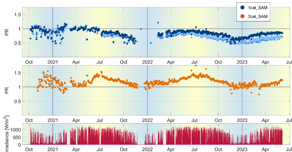
Fig. 4 Long-term outdoor data for \sim 2.5 years of continuous operation of laminated PSCs under MPP tracking in Berlin. The changes in the normalized performance show a periodic pattern with higher PR during the summer period. The bottom panel shows the irradiance during the corresponding outdoor experiments.
