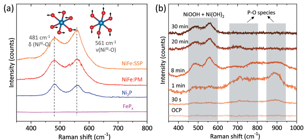
Figure 4. a) Quasi-in-situ Raman spectra of the four different samples (Figure 1) on FTO after 24 hours of OER-CP at 10 \text{ mA cm}^{-2} and subsequent freeze-quenching at 1.53 V_{\text{RHE}} . The two typical vibrations for layered nickel (oxy)hydroxides are marked as grey dashed lines and visualized with the two octahedra (see Figure S32 (Supporting Information) for the spectrum of \text{FeP}_x during OER). b) Quasi-in-situ Raman spectra of NiFe:SSP/FTO film recorded at different times at 1.50 V_{\text{RHE}} to track the time-dependent reconstruction of the transition metal phosphides into nickel(-iron) oxyhydroxides and electrolyte soluble phosphate species.
