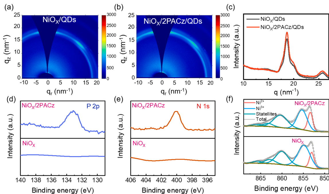
Fig. 2. 2D GIXRD patterns of QDs on (a) \text{NiO}_x and (b) \text{NiO}_x/\text{2PACz} films. (c) Azimuthally integrated 1D plots along the out-of-plane direction. XPS spectra of \text{NiO}_x and \text{NiO}_x/\text{2PACz} surface on ITO for (d) P 2p, (e) N 1s, and (f) Ni 2p.
