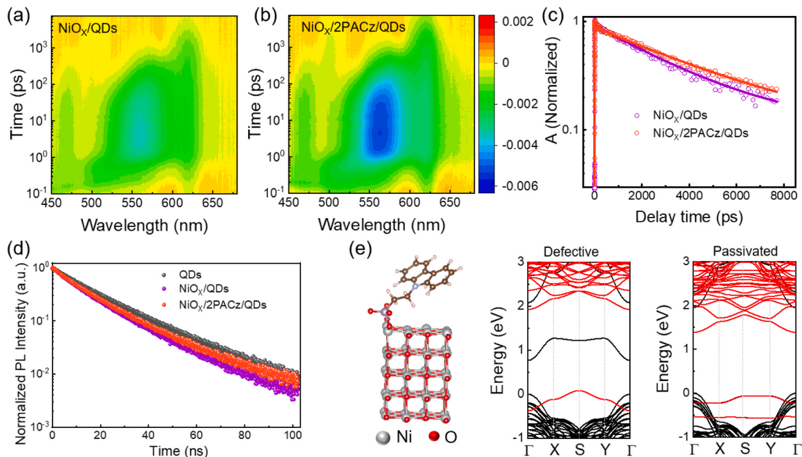
Fig. 4. TA response of (a) \text{NiO}_x/\text{QDs} and (b) \text{NiO}_x/2\text{PACz}/\text{QDs} films. (c) TA delay at a specific wavelength. (d) TRPL decay for the pristine QDs, \text{NiO}_x/\text{QDs} , and \text{NiO}_x/2\text{PACz}/\text{QDs} films deposited on quartz substrates. (e) First-principles simulation of passivation effect of 2\text{PACz} on \text{NiO}_x ( \text{V}_\text{O} ) surfaces.
