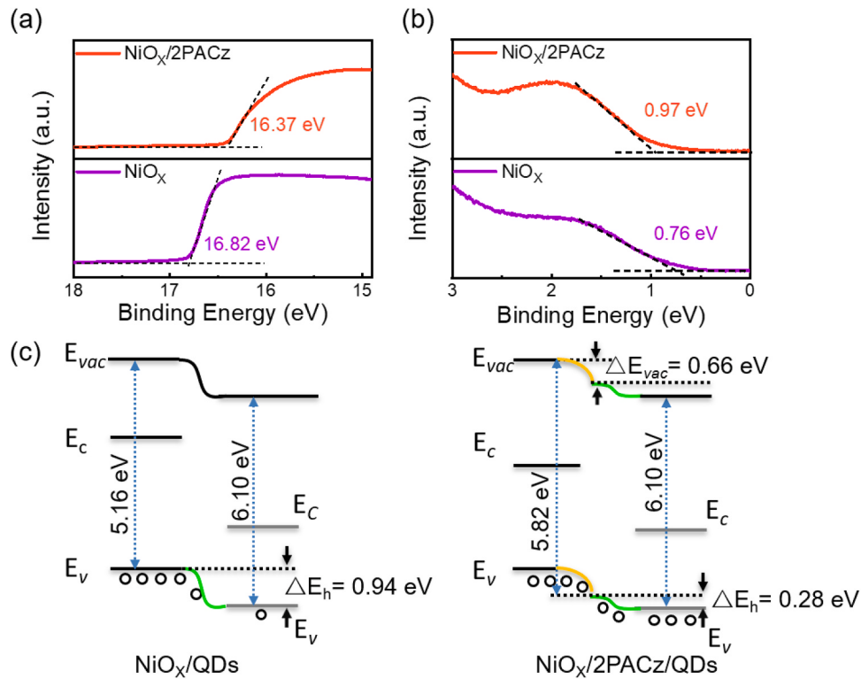
Fig. 3. UPS spectra of \text{NiO}_x and \text{NiO}_x/2\text{PACz} on ITO. (a) the secondary electron cutoff and (b) valence-band edge region. (c) Schematic illustration of energy level alignment at the \text{NiO}_x/\text{QDs} interface (left) and 2\text{PACz} -modified- \text{NiO}_x/\text{QDs} interface (right).
