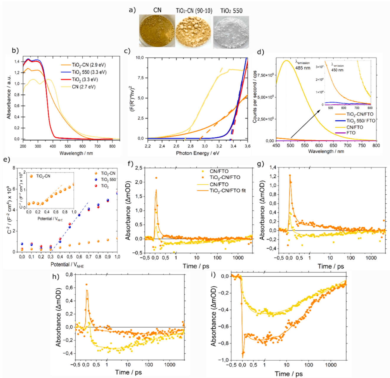
Fig. 3. a) picture of the material powders color of the hybrid cn-tio 2 composite and the two references: CN and calcined TiO 2 . b) UV-vis spectra and c) Tauc plot of CN-TiO 2 composite, TiO 2 550, TiO 2 , and CN samples. d) Steady-state PL spectra of the powder thin film at 400 nm excitation. e) Mott-Schottky plot. Comparison of the TA decays of the CN-TiO 2 composite and CN reference excited at 400 nm at monitoring wavelengths of f) 500 nm, g) 600 nm, h) 700 nm, and i) 1000 nm (excitation density 0.1 mJ/cm 2 ).
