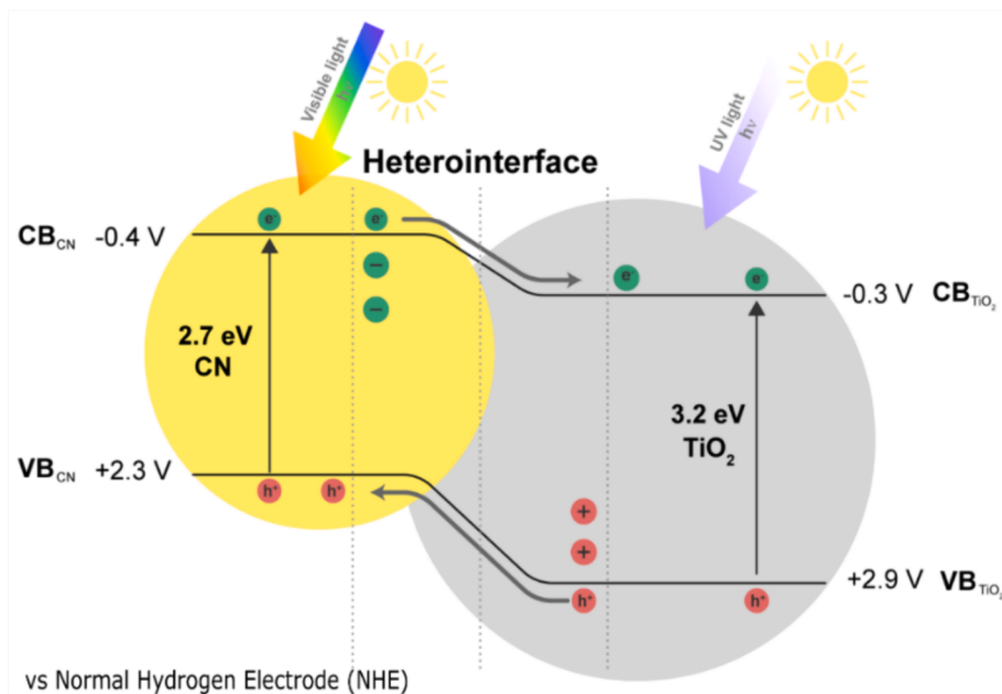
Fig. 1. Heterointerface from coupling CN and TiO_2 with their respective band gaps, CB, and VB edges, and charge carrier transfer possibilities, as postulated for heterojunction type II staggered.
