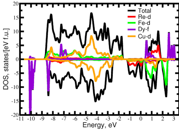
Fig. 6. Total and partial densities of states (DOS) as obtained in the GGA+U+SOC calculations. The Fermi level is set to zero.
