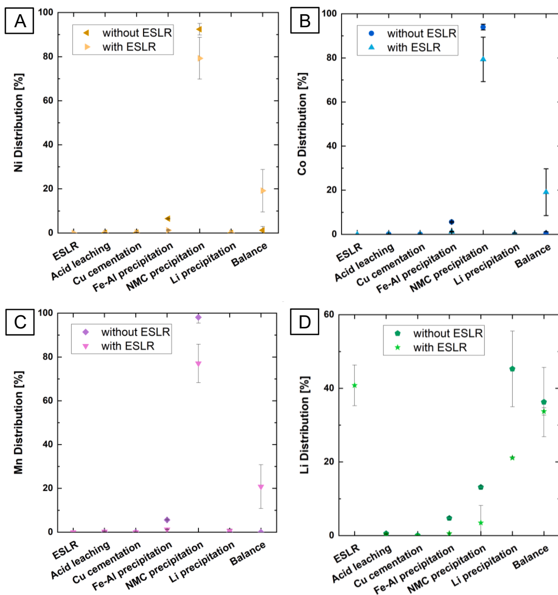
Fig. 3. Comparison of the elemental distribution in the routes with and without ESLR for A: Ni, B: Co, C: Mn, and D: Li.
