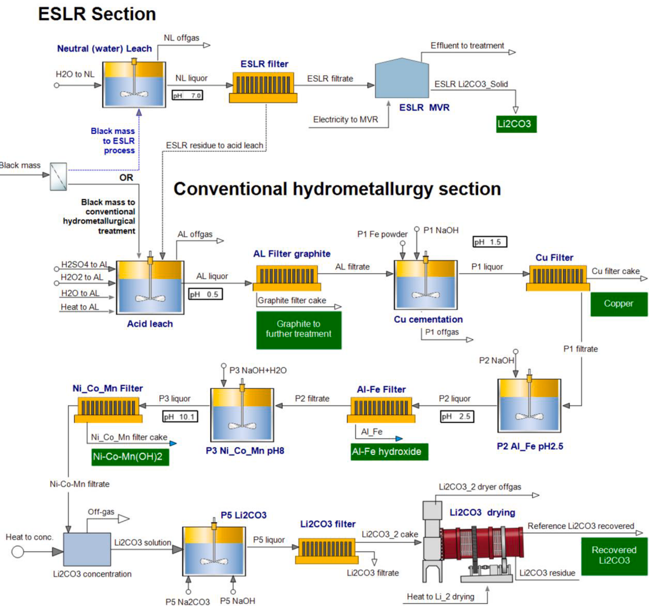
Fig. 2. The process flowsheet from HSC Sim for hydrometallurgical treatment with and without ESLR.
