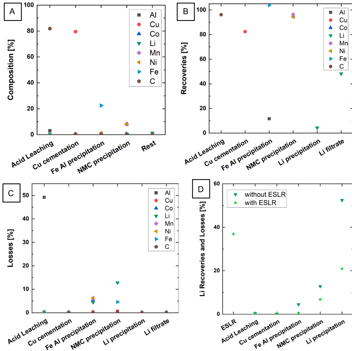
Fig. A1. A: Composition of filter cakes; B and C: recoveries and losses of the different elements in the different process steps of the recycling process; D: Comparison of Li recoveries of the recycling process without and with ESLR
