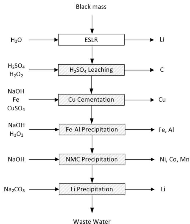
Fig. 1. Grey part: hydrometallurgical battery recycling process according to Wang and Friedrich (reference route); each step includes a filtration step (Wang and Friedrich, 2015); white part: process optimization.
