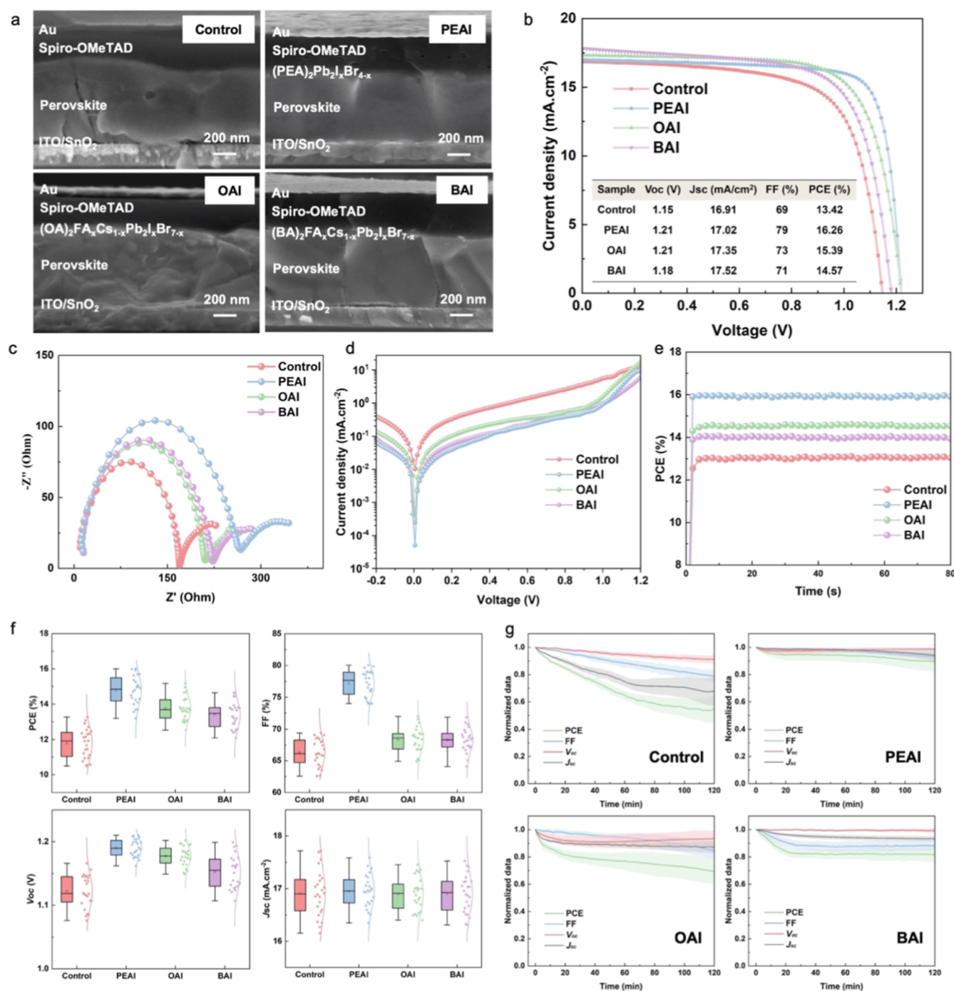
Figure 4. (a) SEM cross-sectional images, (b) champion device J – V curves, (c) electrochemical impedance spectroscopy (EIS) Nyquist plot under light illumination with V_{oc} bias, (d) dark state J – V curves, (e) stabilized power output (SPO), (f) photovoltaic parameters distribution, and (g) temporal evolution of PCE, J_{sc} , V_{oc} , and FF values after 120 min continuous illumination under a nitrogen atmosphere at room temperature of the solar cell device without surface passivation and devices with PEAI, OAI, and BAI passivation.
