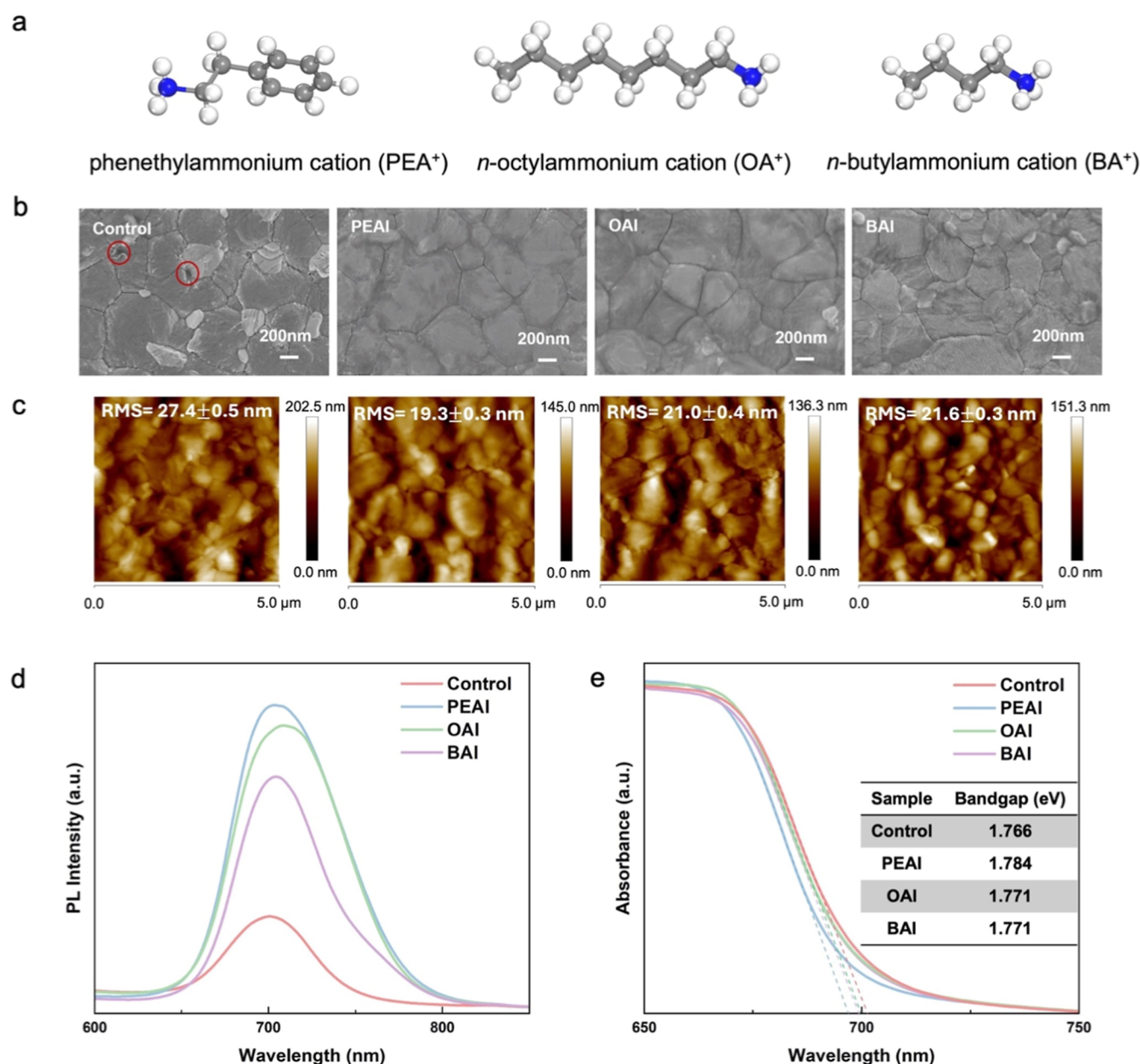
Figure 2. (a) Molecular structures of the three surface passivation materials used. (b) Top-view SEM images, (c) AFM topography images, (d) steady photoluminescence (PL) spectra, and (e) UV-vis optical absorption spectra of pristine perovskite film without surface passivation and films with PEAI, OAI, and BAI passivation. Surface defects are marked by red circles.
