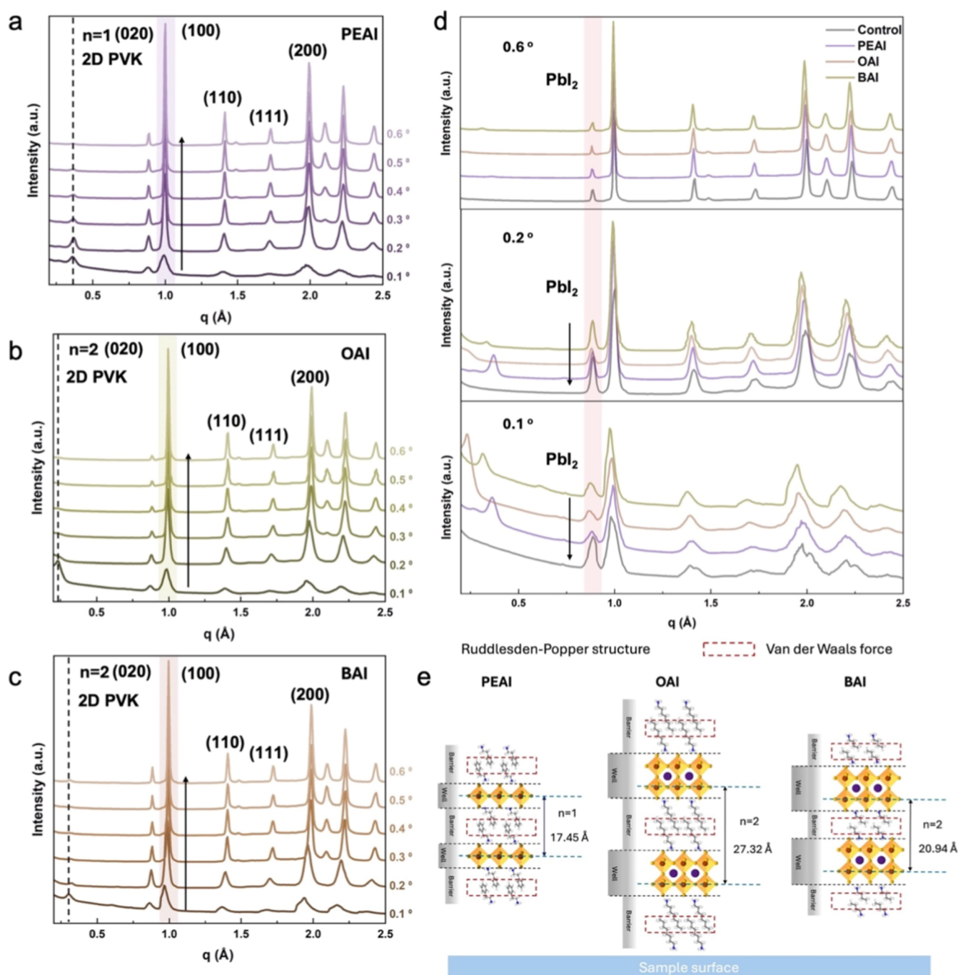
Figure 3. Pseudo XRD spectra (0.1°–0.6° incident angles) of perovskite films with (a) PEAI, (b) OAI, (c) BAI surface passivation. (d) Pseudo XRD spectra (0.1°, 0.2°, and 0.6° incident angles) of perovskite films with and without surface passivation. (e) Schematic representation of the d -spacing of the dominant crystallized plane and quantum well structure of a 2D perovskite layer parallel to the sample surface.
