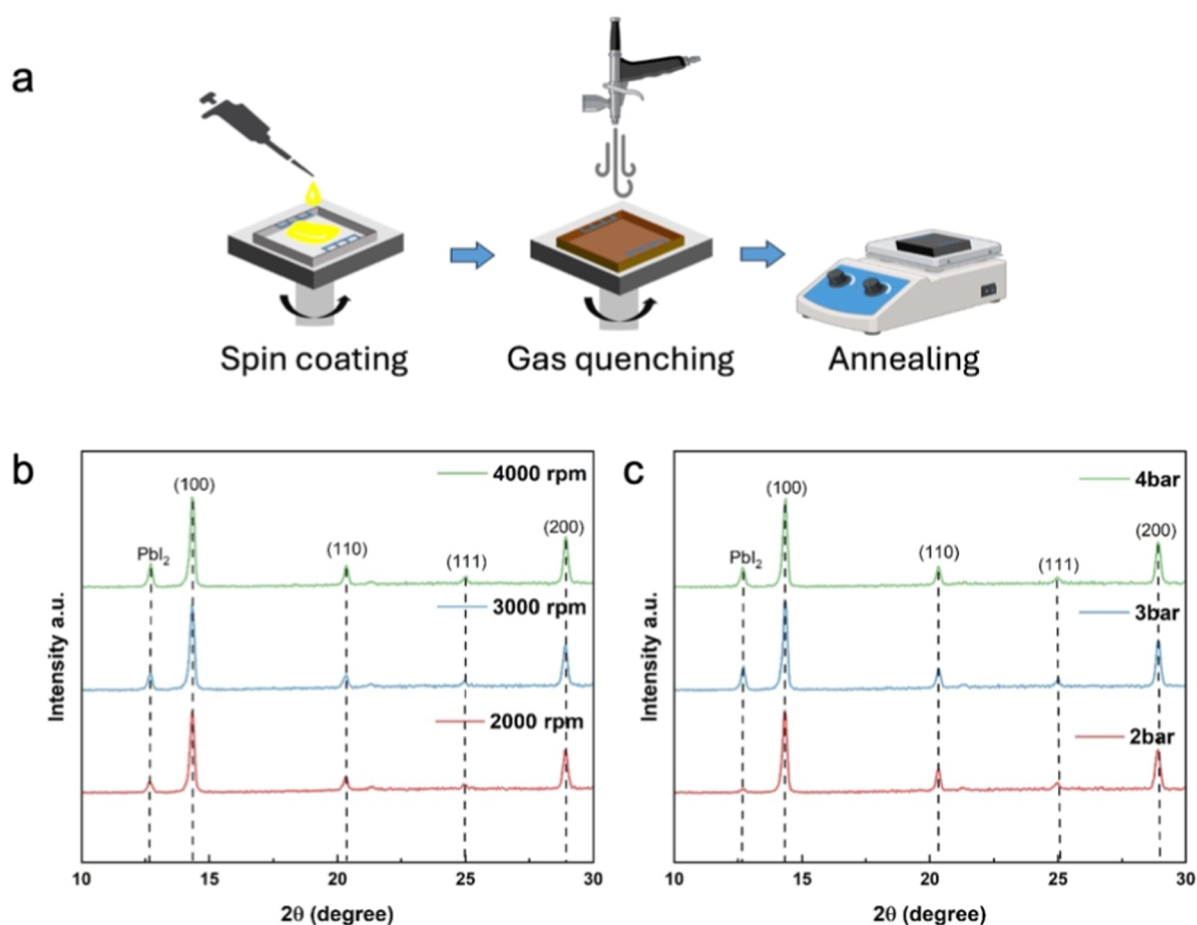
Figure 1. (a) Schematic drawing of the gas quenching process applied during film fabrication via spin-coating. XRD spectra of perovskite films fabricated by gas quenching with (b) different spin coating speeds (2000 rpm, 3000 rpm, 4000 rpm) at a fixed gas flow pressure of 2 bar, and (c) different gas flow pressures (2 bar, 3 bar, 4 bar) at a fixed spin coating speed of 2000 rpm.
