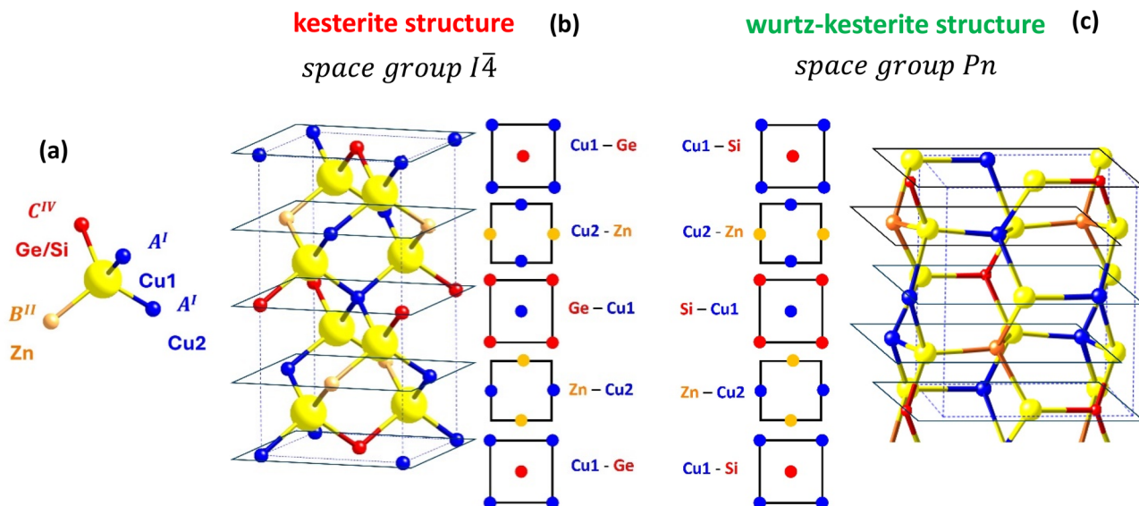
Fig. 1 (a) The anion tetrahedrally coordinated by the cations – the building block of both structures; (b) Cu 2 ZnGeSe 4 in the kesterite structure with Cu1 on 2a, Cu2 on 2c, Zn on 2d and Ge on 2b sites; (c) Cu 2 ZnSiSe 4 in the wurtz-kesterite structure with Cu1 on 2a 1 , Cu2 on 2a 2 , Zn on 2a 3 and Si on 2a 4 sites.
