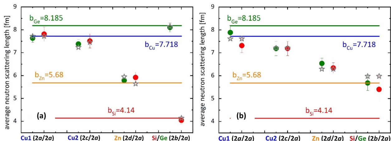
Fig. 6 (a) Average neutron scattering length \bar{b} of the cation sites 2a, 2c, 2d and 2b, assuming a kesterite type structure exemplarily shown for a tetragonal mixed crystal, \text{Cu}_{2.09}\text{Zn}_{1.06}\text{Ge}_{0.95}\text{Se}_4 (green dots) in comparison to the average neutron scattering length \bar{b} of the four 2a cation sites assuming the wurtz-kesterite type structure exemplarily shown for a monoclinic mixed crystal, \text{Cu}_{1.93}\text{Zn}_{0.98}\text{Si}_{1.03}\text{Se}_4 (red dots). Full symbols – experimental average neutron scattering length, stars – calculated average neutron scattering length according to a cation distribution model. (b) The comparison of two cation distributions within a mixed crystal in the structural transition region, \text{Cu}_{2.10}\text{Zn}_{1.03}\text{Ge}_{0.42}\text{Si}_{0.54}\text{Se}_4 , containing two structural phases (kesterite and wurtz-kesterite) with the same chemical compositions (the symbol designations are the same as in (a)).
