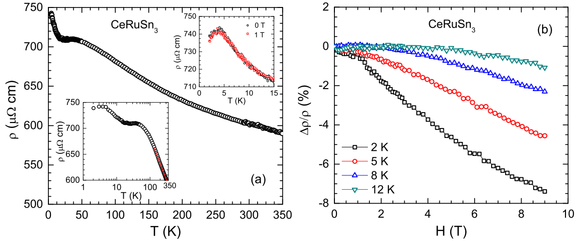
Figure 3. (a) Electrical resistivity \rho of \text{CeRuSn}_3 as a function of temperature T in 2 \text{ K} \leq T \leq 350 \text{ K} measured in applied field H = 0 . Upper inset: Low- T \rho(T) data at H = 0 and 1.0 \text{ T} . Lower inset: \rho(T) data plotted on a semi-logarithmic scale. The red solid line is a fit of \rho(T) data by \rho(T) = \rho_0 - c_K \ln T for 200 \text{ K} \leq T \leq 350 \text{ K} . (b) \rho as a function of H , plotted as magnetoresistance \Delta\rho(H)/\rho(0) for the indicated temperatures of 2, 5, 8 and 12 K.
