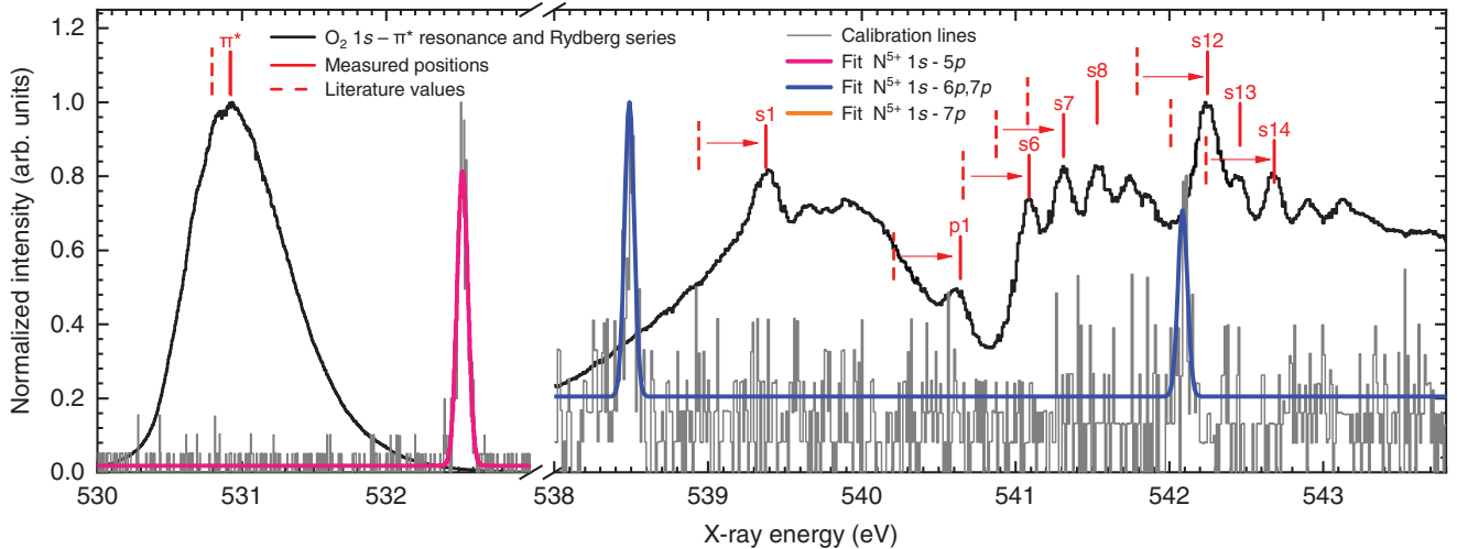
FIG. 3. Recalibration of the O_2 soft x-ray absorption spectrum by simultaneously measuring K_\delta ( 1s-5p ), K_\epsilon ( 1s-6p ), and K_\zeta ( 1s-7p ) transitions in He-like N^{5+} as energy references. Positions of spectral features in O_2 from the literature [21,37] (dashed red vertical markers) are compared with our measurements (full red vertical markers), clearly showing the energy offset (see Table I). The vertical scales are different for the two spectral regions shown.
