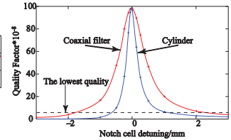
Figure 6: Quality factor of the cavity with the shortcut at the coaxial filter end
