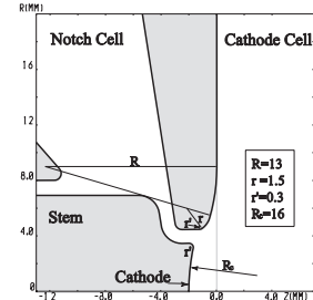
Figure 3: Upgraded geometry of the cathode insert.
