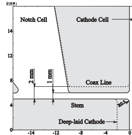
Figure 2: Initial cathode insert geometry [3, 4, 5].
