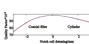
Figure 5: Quality factor of the cavity with unloaded coaxial filter.
