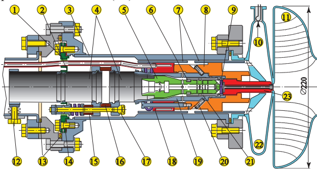
Figure 1: The sketch of the upgraded cathode insert.
