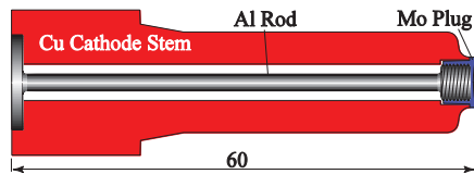
Figure 4: The cathode stem (mm scale).
