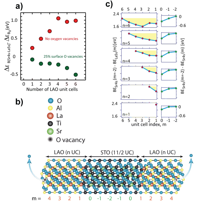
FIG. 5. (color online). a) The n -dependence of the potential in the \text{LaAlO}_3 expressed via the relative changes in the La 5s shallow core level binding energy extracted from the DFT calculations for vacancy free and oxygen deficient LAO/STO systems described in the text. Points describing a positive slope reflect a trend to decreasing La core level binding energy. b) The 2 \times 2 lateral supercell used in the DFT calculations. Oxygen vacancies (25%) were located in the outermost \text{AlO}_2 layers. c) Layer-by-layer data from the DFT calculations for the system shown in panel (b). The right hand panels show the n -dependence of the energetics in the STO substrate and the left hand panels show the evolution of the energies across the \text{LaAlO}_3 films. The yellow shading indicates regions with LAO potentials such that the La core levels move to higher binding energy, opposite to the direction of the in-built potential scenario.
