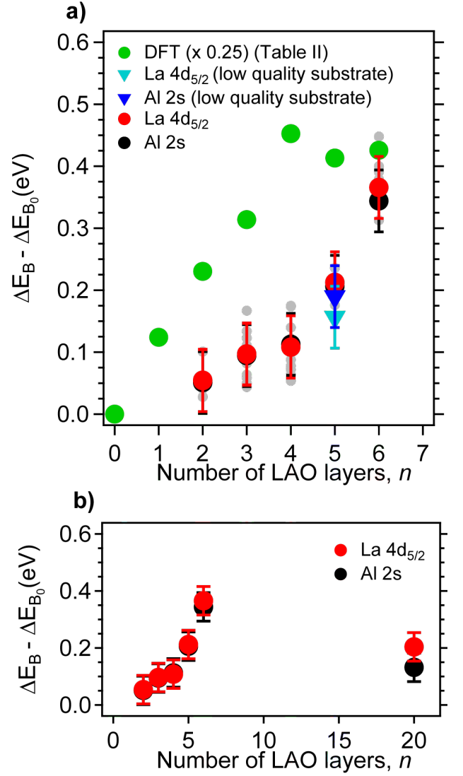
FIG. 3. (color online) Evolution of the energetics in the LaAlO _3 overlayer tracked using the La 4d and Al 2s core level binding energies vs. LaAlO _3 thickness, n . a) Data up to n = 6 . To indicate the spread in energy shifts encountered, in addition to the main data-points (see legend), the smaller grey symbols show energy shift data from all experiments we conducted on STO/LAO interface samples, including using Al:K _{\alpha} radiation, and using samples from other thin film growth batches. For comparison with experiment, one fourth of the expected core level shift based on DFT calculations for a vacancy free interface is also shown as an average weighted by the inelastic mean-free path length in HAXPES. The results of these calculations are also shown in Table II. b) Energy shift data including n = 20 .
