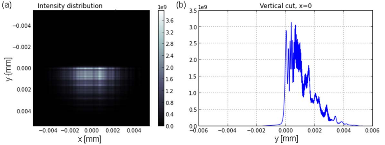
Fig. 7: (a) The profile of the reflected beam 130 m from the beam-splitter. (b) Vertical cut through the beam-profile at x = 0 mm.
