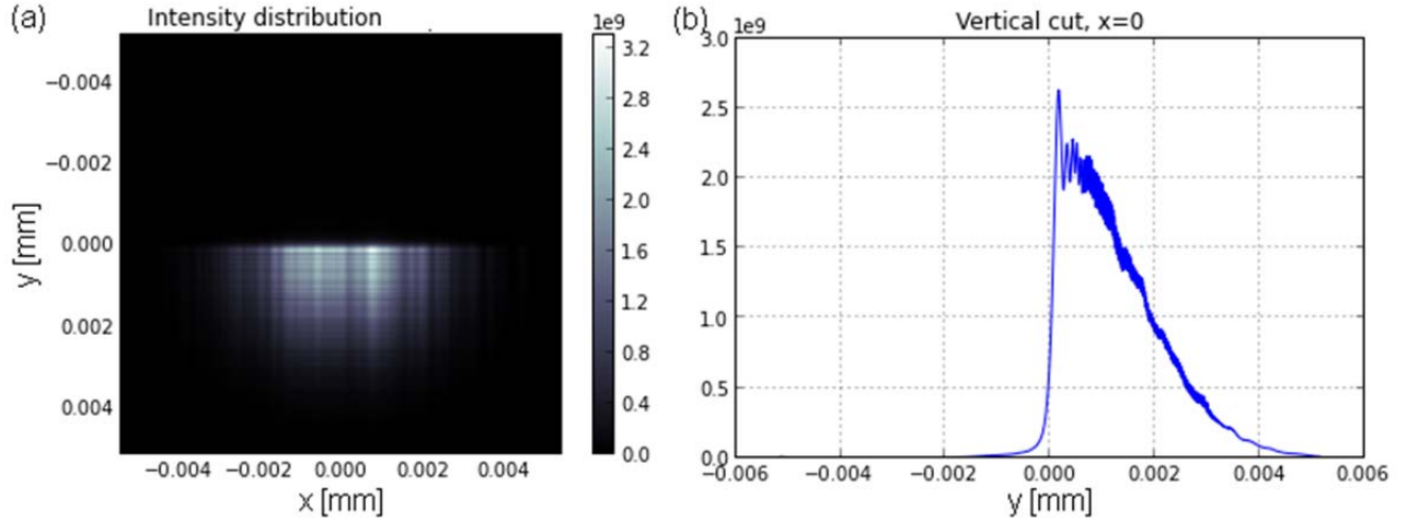
Fig. 8: A similar simulation as shown in Fig. 7, with an improved substrate (height-error 3 nm peak-to-valley).
