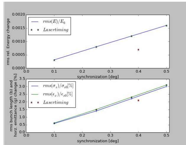
Figure 3: Central energy (top) and the emittance and bunch length (bottom) as a function of the synchronization. Red star: contribution of the laser timing.
