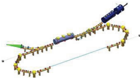
Figure 1: Scheme of the bERLinPro ERL with the injector section on the top right of the picture.
