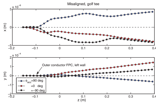
Figure 5: Kick induced by a misaligned twin coupler for a 5 ps bunch by PIC calculations. The position of the coupler by the opening of the outer conductor is marked by the black arrow.
