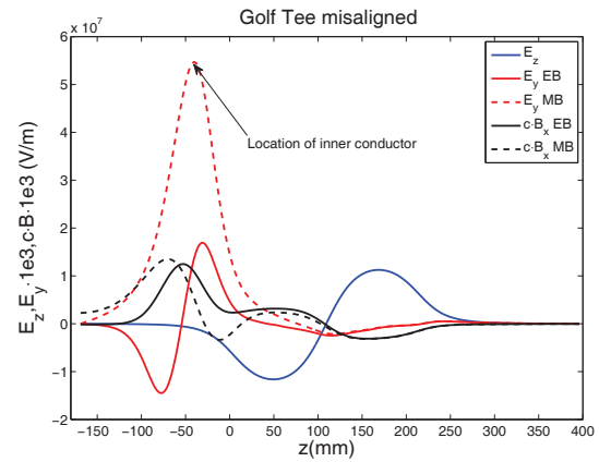
Figure 4: On-axis longitudinal and transverse field components for a misaligned "golf tee" coupler pair with EB and MB conditions.
