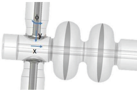
Figure 3: Misalignment scenarios studied for the modified KEK coupler as attached to the 2-cell SRF booster cavity. The upper inner conductor is shifted with respect to the opposing FPC port in x and y and (for the "golf tee" only) rotated in \phi .
