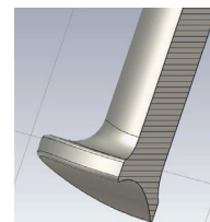
Figure 2: New "golf tee" shaped coupler tip to increase the coupling strength and reduce coupler kick effects.
