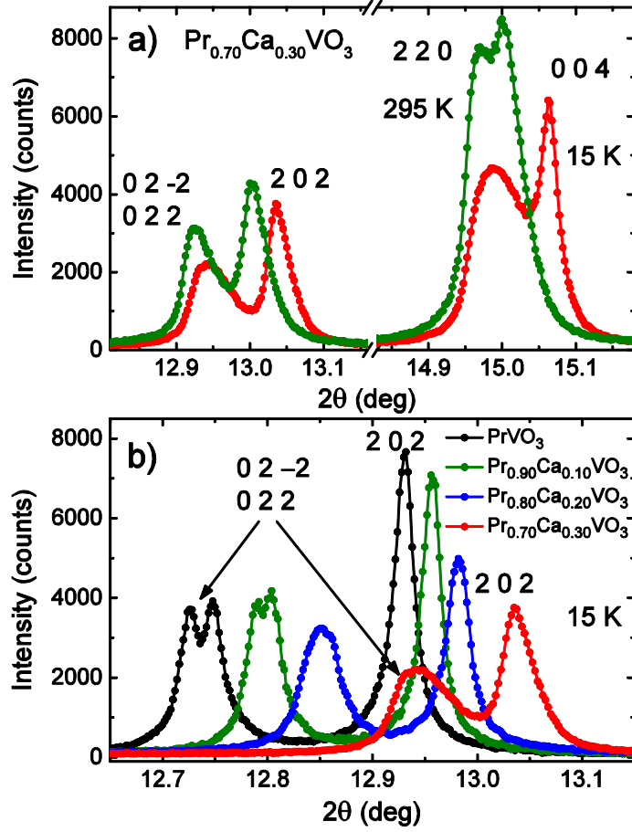
FIG. 4. (color online) Sections of synchrotron diffraction patterns of \text{Pr}_{1-x}\text{Ca}_x\text{VO}_3 . (a) Comparison of the peak profiles of \text{Pr}_{0.70}\text{Ca}_{0.30}\text{VO}_3 measured at 15 and 295 K. At 15 K a strongly anisotropic peak broadening was observed, where the linewidth (HWHM) of the reflection 220 shows the strongest increase. (b) Evolution of the monoclinic peak splitting in \text{Pr}_{1-x}\text{Ca}_x\text{VO}_3 with increasing Ca doping. For the insulating vanadates with x = 0, 0.10, 0.20 the orthorhombic 022 reflection splits into the monoclinic reflections 022 and 02-2, respectively. With increasing Ca content the monoclinic distortions are continuously weakened and disappear in the metallic state. However, the reflection pair 022/02-2 shows an asymmetrically broadened peak profile.
