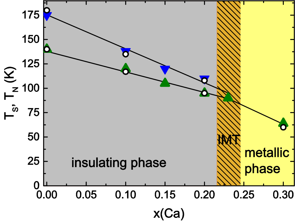
FIG. 2. (color online) Change of the structural and magnetic phase transitions in the system \text{Pr}_{1-x}\text{Ca}_x\text{VO}_3 as a function of the doping level x . With increasing Ca content an insulator-metal transition occurs at x = 0.23 , which causes the melting of the G -type orbital order. The structural and magnetic phase transitions were determined earlier from specific heat (blue triangles) and magnetization measurements (green triangles), respectively. 10 In the present work both types of phase transitions were reinvestigated by single-crystal neutron diffraction (open black circles). Note that the error bars correspond to the size of the symbols. The bold lines are guides to the eye.
