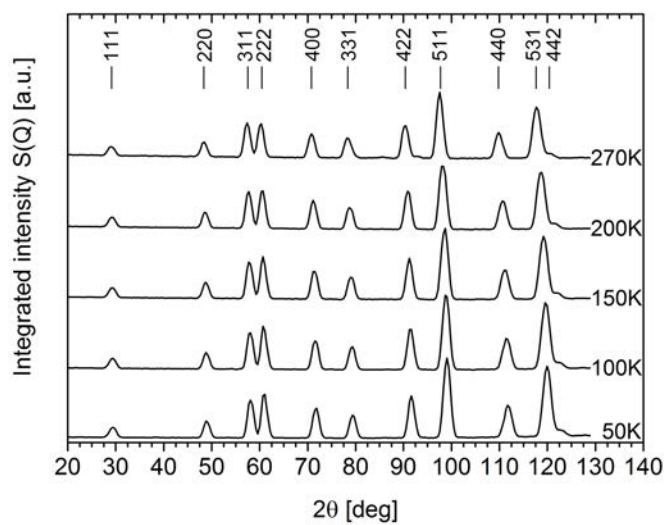
Figure 1: Powder diffractograms of the THF clathrates hydrates recorded at indicated temperatures with the ToF spectrometer IN5@ILL ( \lambda_0 = 5 \text{ \AA} ). The Bragg peaks are indexed in the type II clathrate structure (i.e space group Fd3m with a \approx 17.2 \text{ \AA} ).
