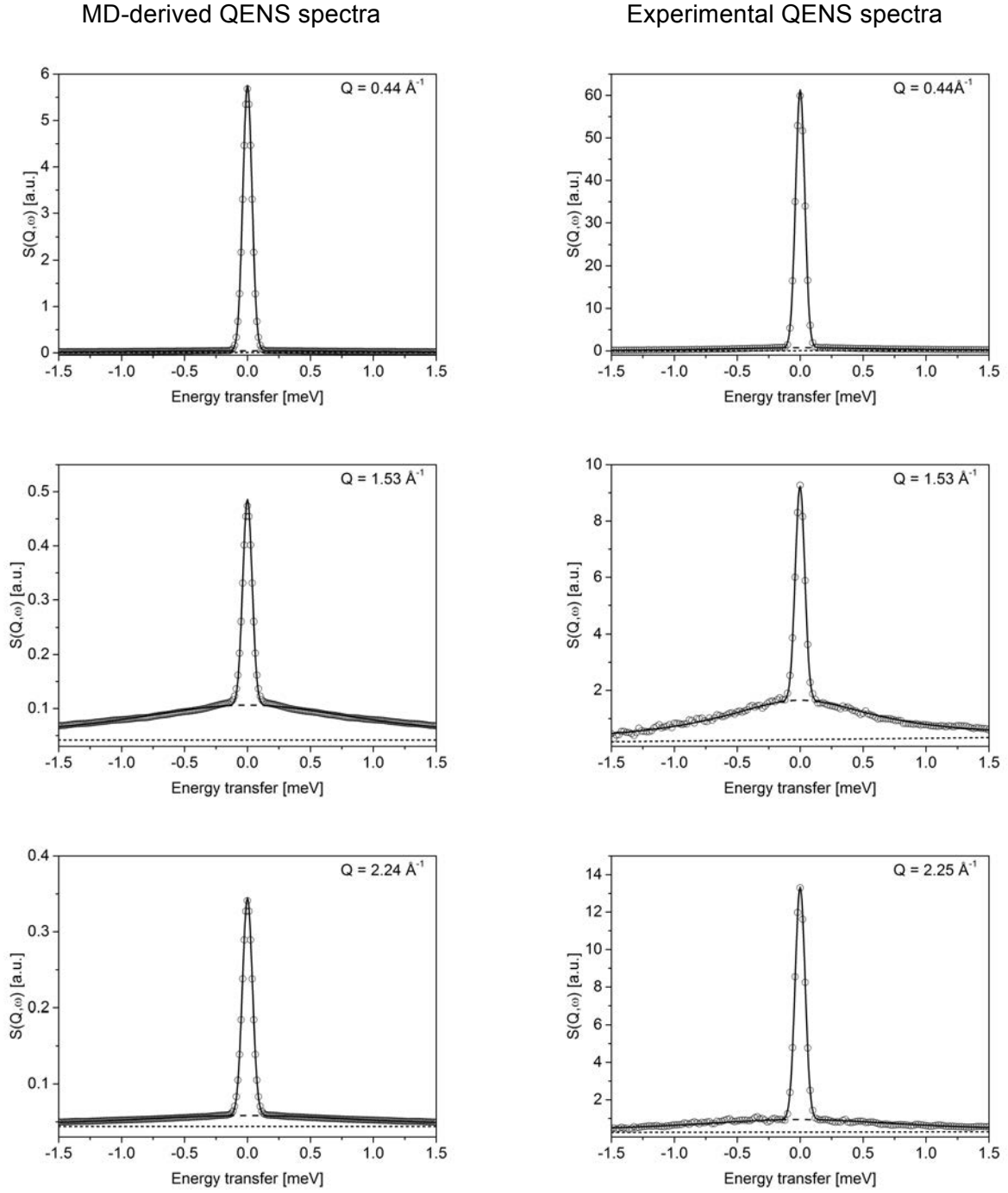
Figure 4: MD-derived (left hand) and experimental (right hand) neutron scattering laws (points) of the THF clathrate hydrates at 270K (energy resolution \Delta E \sim 90 \mu\text{eV} for an incident wavelength \lambda_0 = 5 \text{ \AA} ). The thick continuous line is the fitted scattering laws according to equation (6). The dashed lines represents the fitted quasielastic components and the dotted lines, scattering backgrounds.
