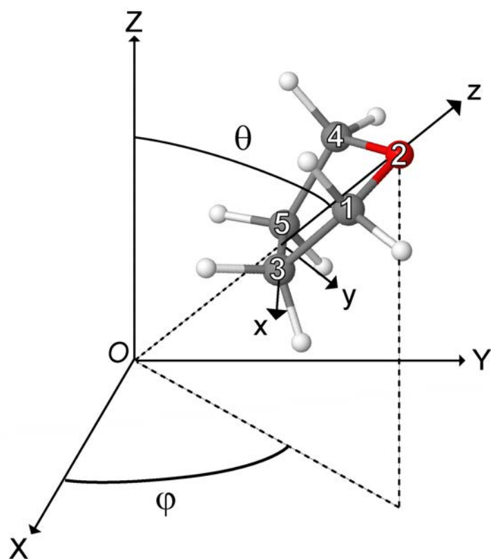
Figure 2: Representation of THF molecular frame (Cxyz) as well as the polar ( \theta ) and azimuth ( \phi ) angles with respect of the MD box reference frame (OXYZ).
