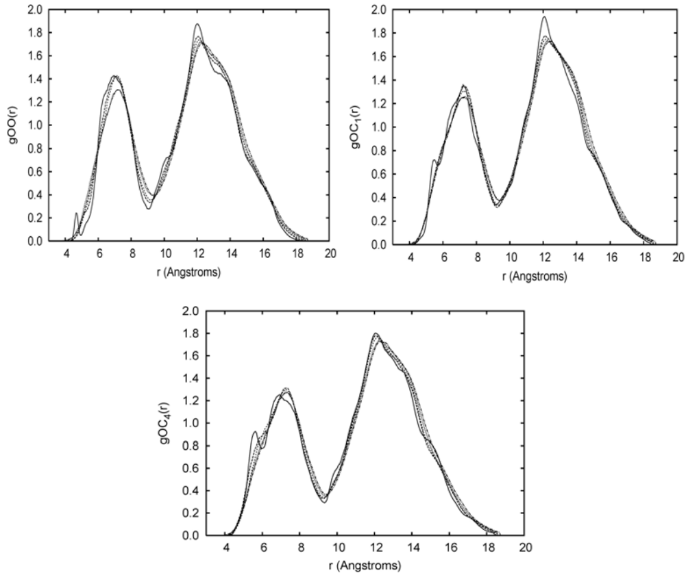
Figure S3: Pair distribution functions g_{OO}(r) and g_{OC}(r) for THF obtained from MD simulations at various temperatures as specified in Figure S1.
