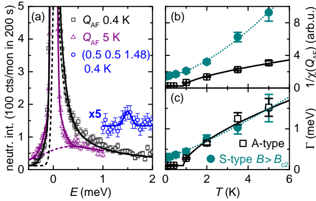
FIG. 1. (a) Spectra of \text{CeCu}_2\text{Si}_2 at 0.4 K (black) and 5 K (purple), measured at Q_{\text{AF}} = (0.215 \ 0.215 \ 1.48) ; solid black/purple lines show total fit functions, dashed black/purple lines show inelastic magnetic contribution, which was fitted with a Bose-weighted Lorentzian function. Shown in blue is a scan at the magnetic zone boundary Q = (0.5 \ 0.5 \ 1.48) at 0.4 K with a Gaussian fit; these data have been magnified by a factor of 5. (b) Fitted inverse susceptibility 1/\chi and (c) width \Gamma (full width at half maximum, FWHM) of the inelastic magnetic signal at Q_{\text{AF}} , for our A-type crystal and for the S-type crystal at 1.7 T (taken from reference 23 ). \chi(Q_{\text{AF}}) is normalised to the intensity of the incoherent elastic line 29 . Lines are guides to the eye.
