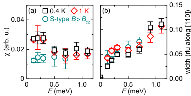
FIG. 3. (a) Susceptibility associated with the constant- E scans, obtained from the integrated intensity over both branches of the dispersion, and further corrected for the Bose temperature factor. The data for the S-type crystal are taken in the normal state at 1.7 T and 60 mK. The same normalisation to the incoherent elastic line has been done as in Fig. 1 29 . (b) Width (FWHM) of the constant- E scans along [110].
