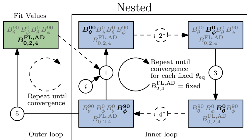
FIG. 4: Flowchart of the nested iterative procedure to extract spin-orbit torques from harmonic measurements. Updated steps in the nested iterative procedure are highlighted as dashed lines (as compared to the conventional procedure). The steps, indicated by the encircled numbers, are explained in the text. The updated quantities are in bold. Note that for each iteration of the outer loop, the conventional procedure in the inner loop converges.
