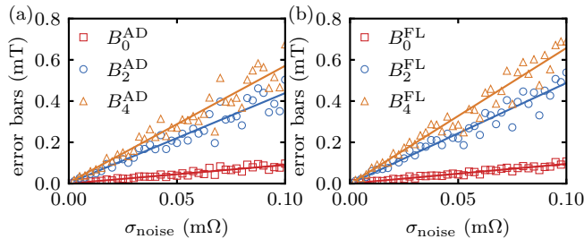
FIG. 6: Error bars of the extracted SOT parameters in the presence of experimental noise \sigma_{\text{noise}} . The simulation input parameters are listed in Tab. II and \sigma_{\text{noise}} was added to the simulated first and second harmonic signals (see Fig. 2, sampled in 1 mT steps). Panels (a) and (b) show the results and linear fits for B_{0,2,4}^{\text{AD}} and B_{0,2,4}^{\text{FL}} , respectively.
