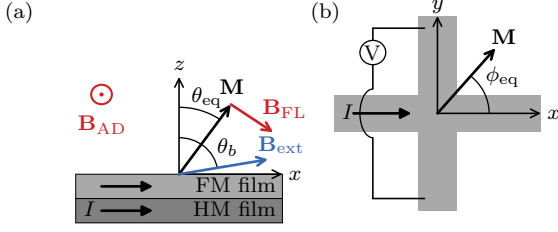
FIG. 1: Geometry and coordinate system. (a) Side view of the Hall bar structure. \mathbf{M} is the magnetization, \mathbf{B}_{\text{ext}} the external applied field. \theta_{\text{eq}} and \theta_b are the azimuthal angles of the magnetization and external applied field from the z -axis, respectively. \mathbf{B}_{\text{AD}} , \mathbf{B}_{\text{FL}} are the effective SOT fields. (b) Top view of the Hall bar structure indicating the in-plane angle \phi_{\text{eq}} of the magnetization, as well as the measurement direction of the transverse voltage.
