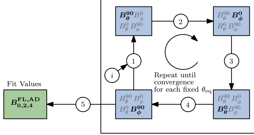
FIG. 3: Flowchart of the conventional iterative procedure to extract spin-orbit torques from harmonic measurements. The steps, indicated by the encircled numbers, are explained in the text. The updated quantities are printed in bold. Note that the fit of the desired torque coefficients is performed only once, after the boxed loop has reached convergence.
