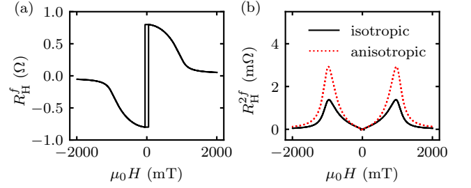
FIG. 2: Expected (a) first harmonic signal R_{\text{H}}^f and (b) second harmonic signal R_{\text{H}}^{2f} , the latter with and without higher order coefficients at \phi_{\text{eq}} = 90^\circ , \theta_b = 88^\circ . For the simulated SOT parameters see Tabs. I and II.
