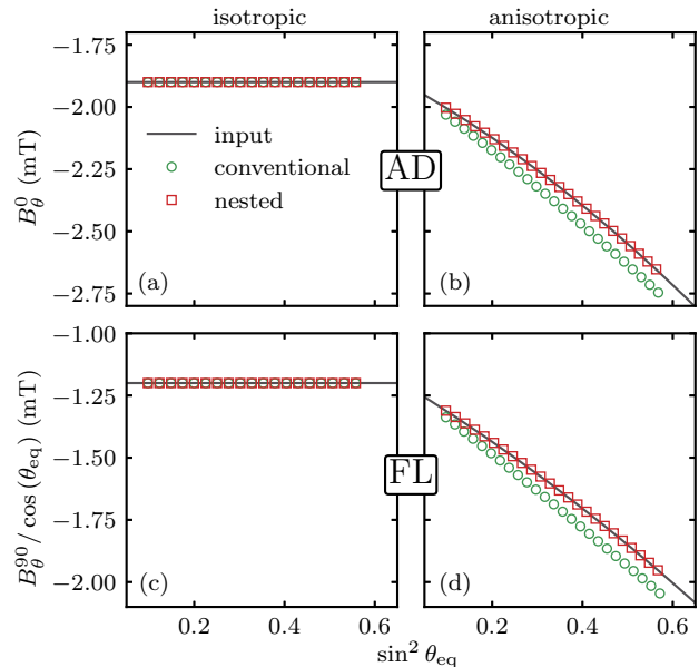
FIG. 5: SOT fields extracted from the conventional and nested iterative analysis as a function of magnetization angle \sin^2 \theta_{\text{eq}} . Figures (a) and (c) show the results for the isotropic SOTs (see parameters in Tab. I). Figures (b) and (d) show the fields extracted from the anisotropic SOT simulation (see Tab. II). The functional dependence expected from the known input parameters is plotted with solid lines. The extracted torque coefficients are listed in the Tabs I and II.
